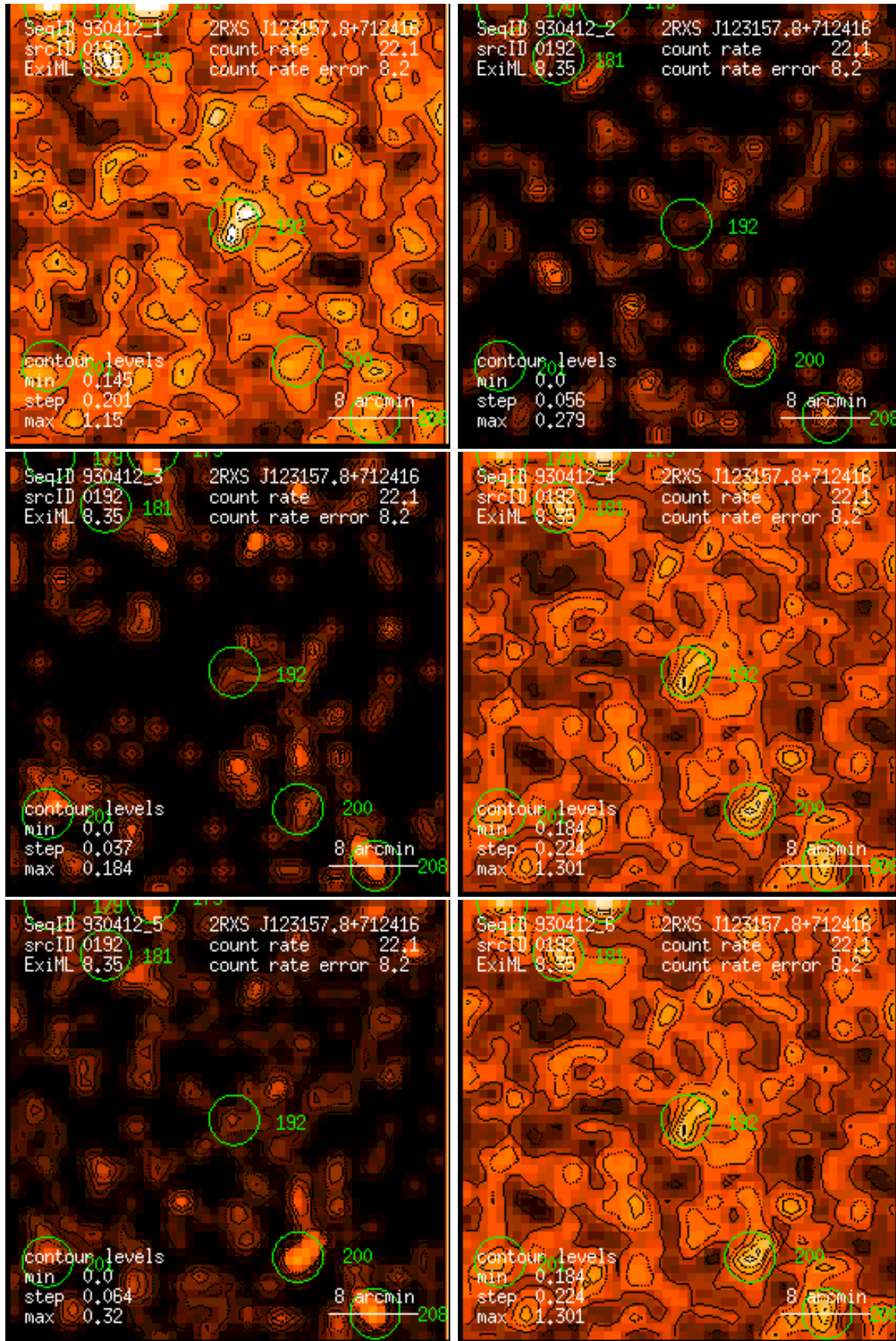
Figure 192: RASS 930412: detection 0192: band rate images, Gaussian filter: (1) PSPC channels 11 – 41, (2) 52 – 90, (3) 91 – 201, (4) 11 – 235, (5) 52 – 201, (6) 11 – 201. Broad band rates in counts/ks. Band rate contour levels in counts/ks/arcmin 2 .
