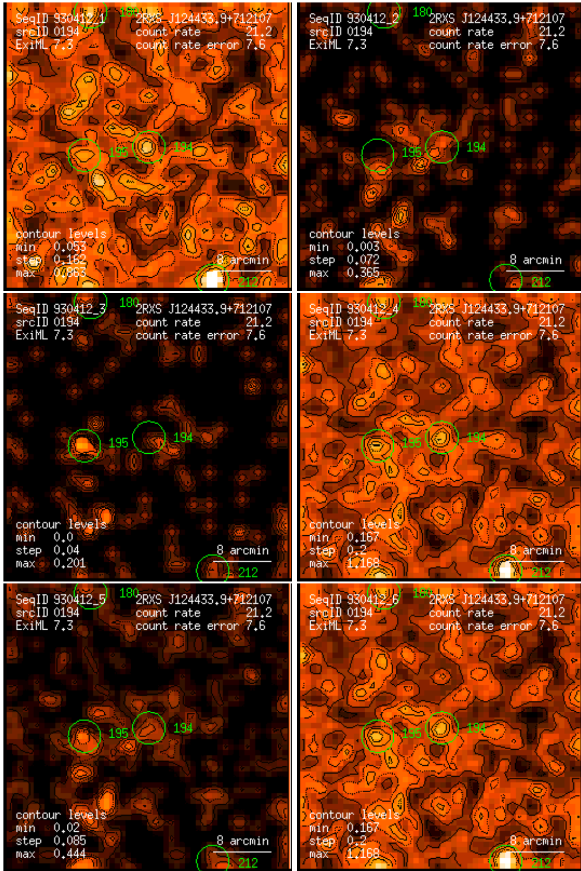
Figure 194: RASS 930412: detection 0194: band rate images, Gaussian filter: (1) PSPC channels 11 – 41, (2) 52 – 90, (3) 91 – 201, (4) 11 – 235, (5) 52 – 201, (6) 11 – 201. Broad band rates in counts/ks. Band rate contour levels in counts/ks/arcmin 2 .
