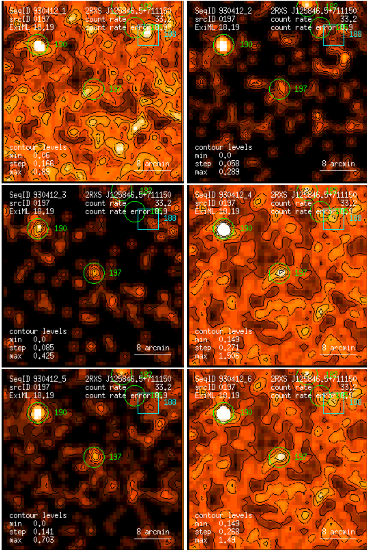
Figure 197: RASS 930412: detection 0197: band rate images, Gaussian filter: (1) PSPC channels 11 – 41, (2) 52 – 90, (3) 91 – 201, (4) 11 – 235, (5) 52 – 201, (6) 11 – 201. Broad band rates in counts/ks. Band rate contour levels in counts/ks/arcmin 2 .
