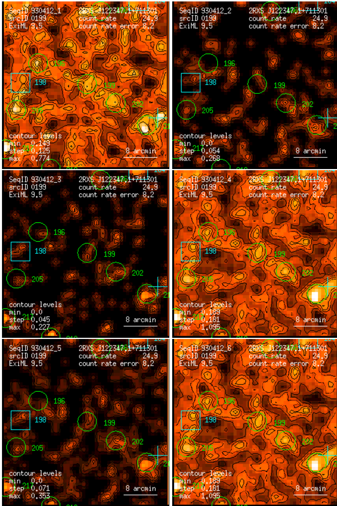
Figure 199: RASS 930412: detection 0199: band rate images, Gaussian filter: (1) PSPC channels 11 – 41, (2) 52 – 90, (3) 91 – 201, (4) 11 – 235, (5) 52 – 201, (6) 11 – 201. Broad band rates in counts/ks. Band rate contour levels in counts/ks/arcmin 2 .
