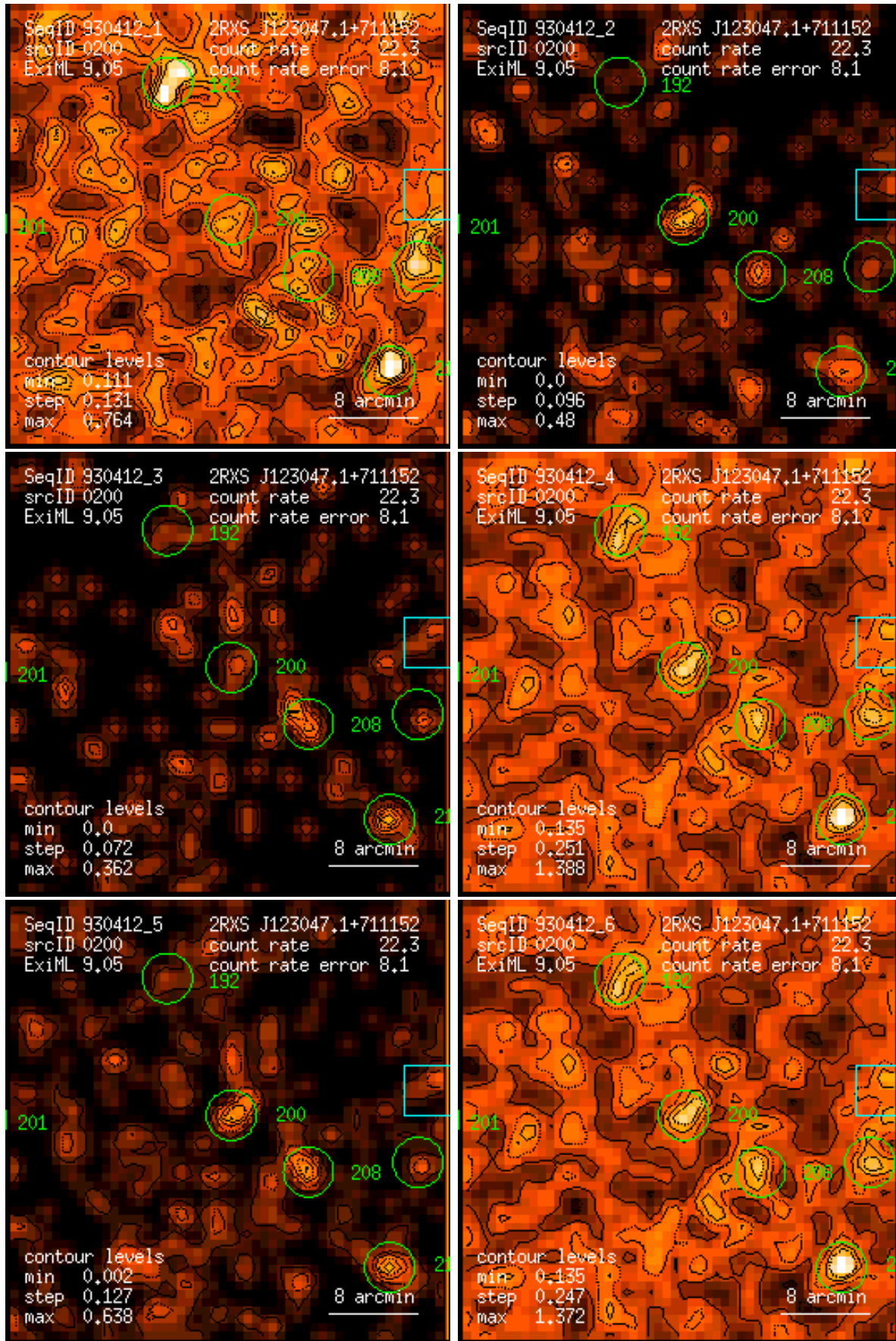
Figure 200: RASS 930412: detection 0200: band rate images, Gaussian filter: (1) PSPC channels 11 – 41, (2) 52 – 90, (3) 91 – 201, (4) 11 – 235, (5) 52 – 201, (6) 11 – 201. Broad band rates in counts/ks. Band rate contour levels in counts/ks/arcmin 2 .
