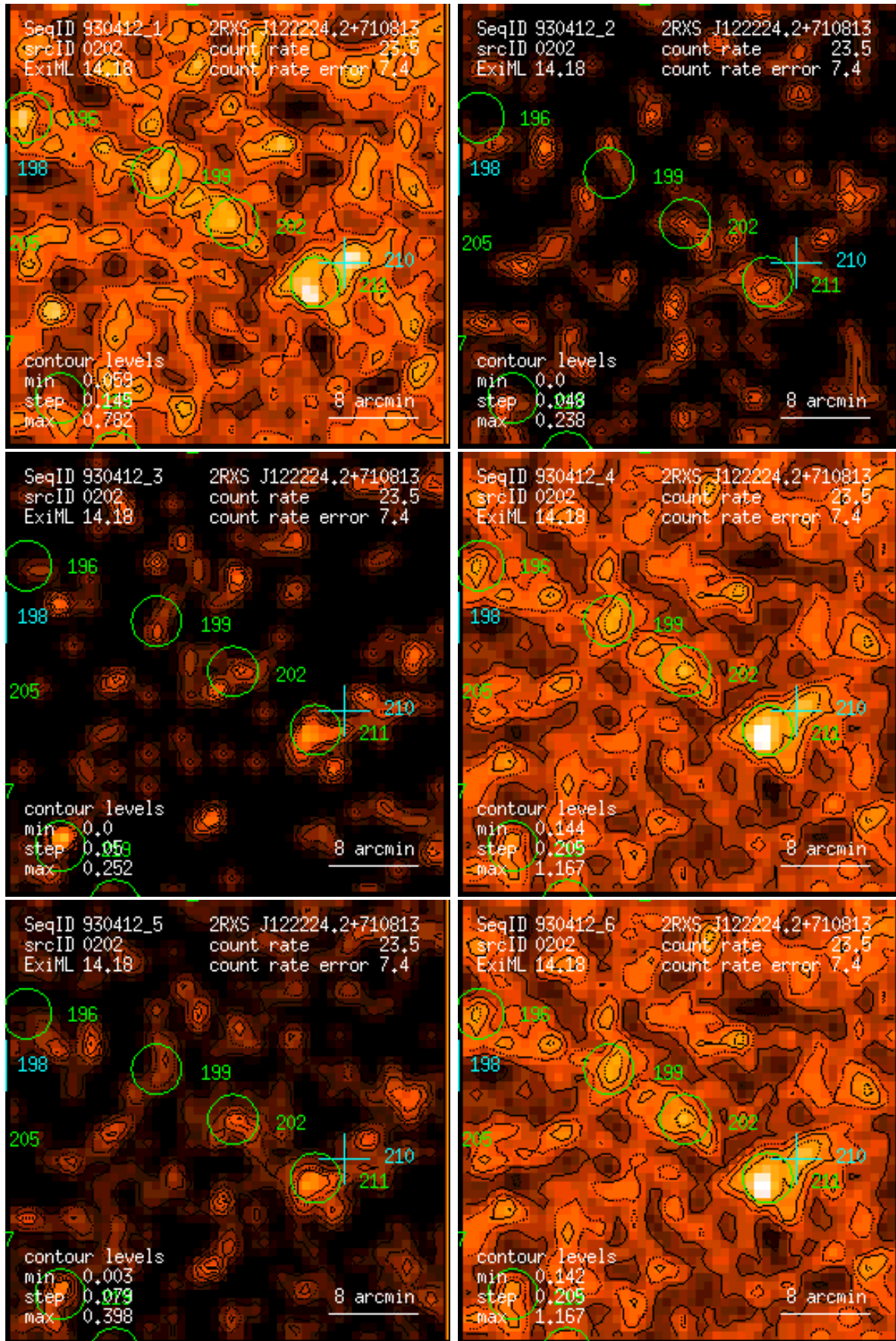
Figure 202: RASS 930412: detection 0202: band rate images, Gaussian filter: (1) PSPC channels 11 – 41, (2) 52 – 90, (3) 91 – 201, (4) 11 – 235, (5) 52 – 201, (6) 11 – 201. Broad band rates in counts/ks. Band rate contour levels in counts/ks/arcmin 2 .
