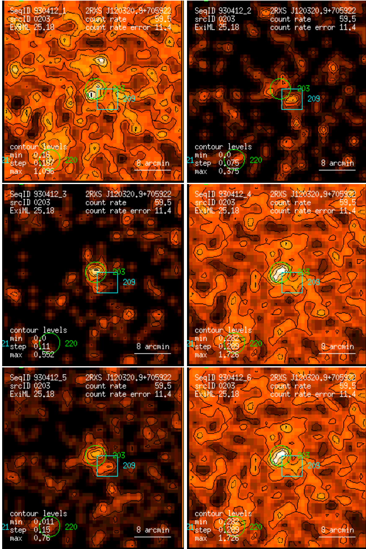
Figure 203: RASS 930412: detection 0203: band rate images, Gaussian filter: (1) PSPC channels 11 – 41, (2) 52 – 90, (3) 91 – 201, (4) 11 – 235, (5) 52 – 201, (6) 11 – 201. Broad band rates in counts/ks. Band rate contour levels in counts/ks/arcmin 2 .
