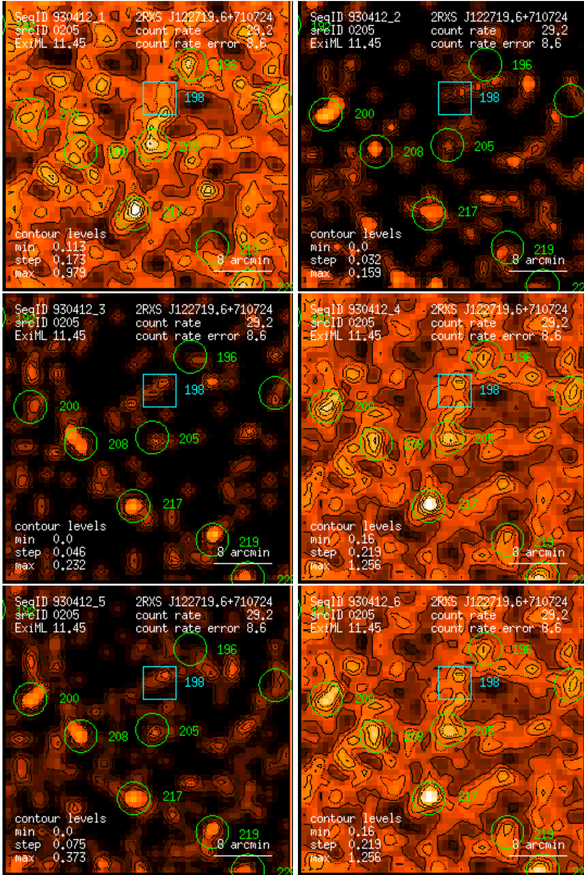
Figure 205: RASS 930412: detection 0205: band rate images, Gaussian filter: (1) PSPC channels 11 – 41, (2) 52 – 90, (3) 91 – 201, (4) 11 – 235, (5) 52 – 201, (6) 11 – 201. Broad band rates in counts/ks. Band rate contour levels in counts/ks/arcmin 2 .
