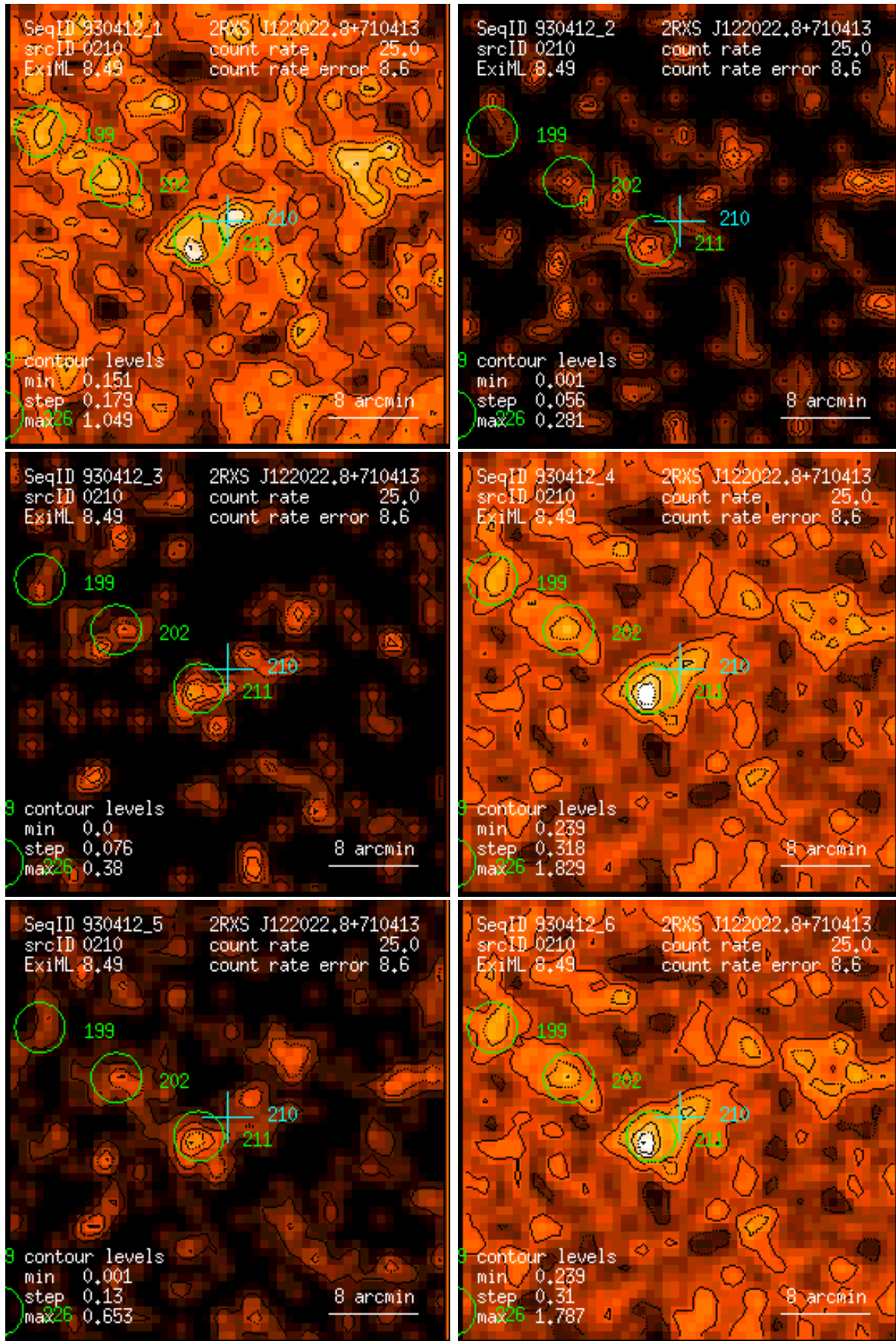
Figure 210: RASS 930412: detection 0210: band rate images, Gaussian filter: (1) PSPC channels 11 – 41, (2) 52 – 90, (3) 91 – 201, (4) 11 – 235, (5) 52 – 201, (6) 11 – 201. Broad band rates in counts/ks. Band rate contour levels in counts/ks/arcmin 2 .
