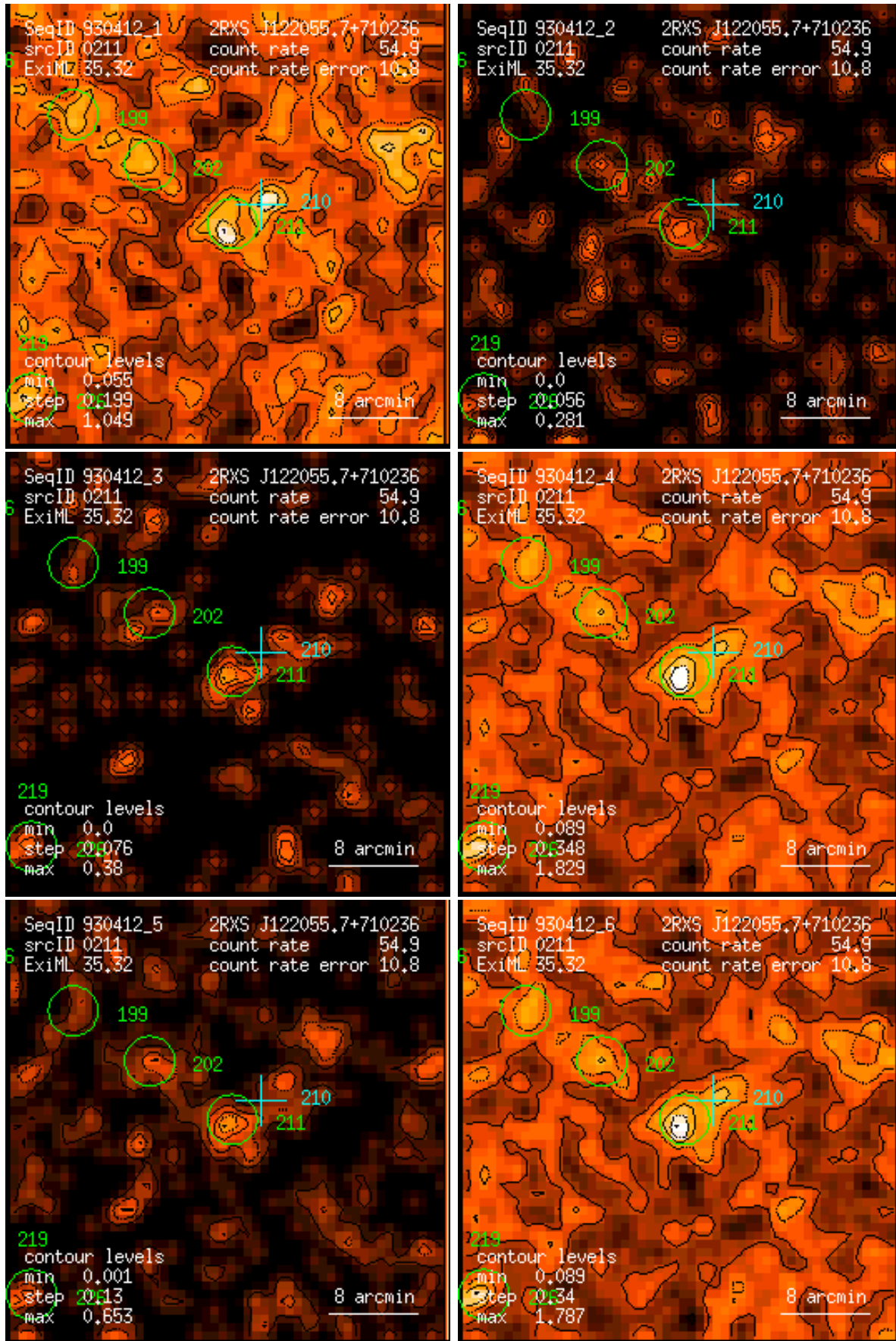
Figure 211: RASS 930412: detection 0211: band rate images, Gaussian filter: (1) PSPC channels 11 – 41, (2) 52 – 90, (3) 91 – 201, (4) 11 – 235, (5) 52 – 201, (6) 11 – 201. Broad band rates in counts/ks. Band rate contour levels in counts/ks/arcmin 2 .
