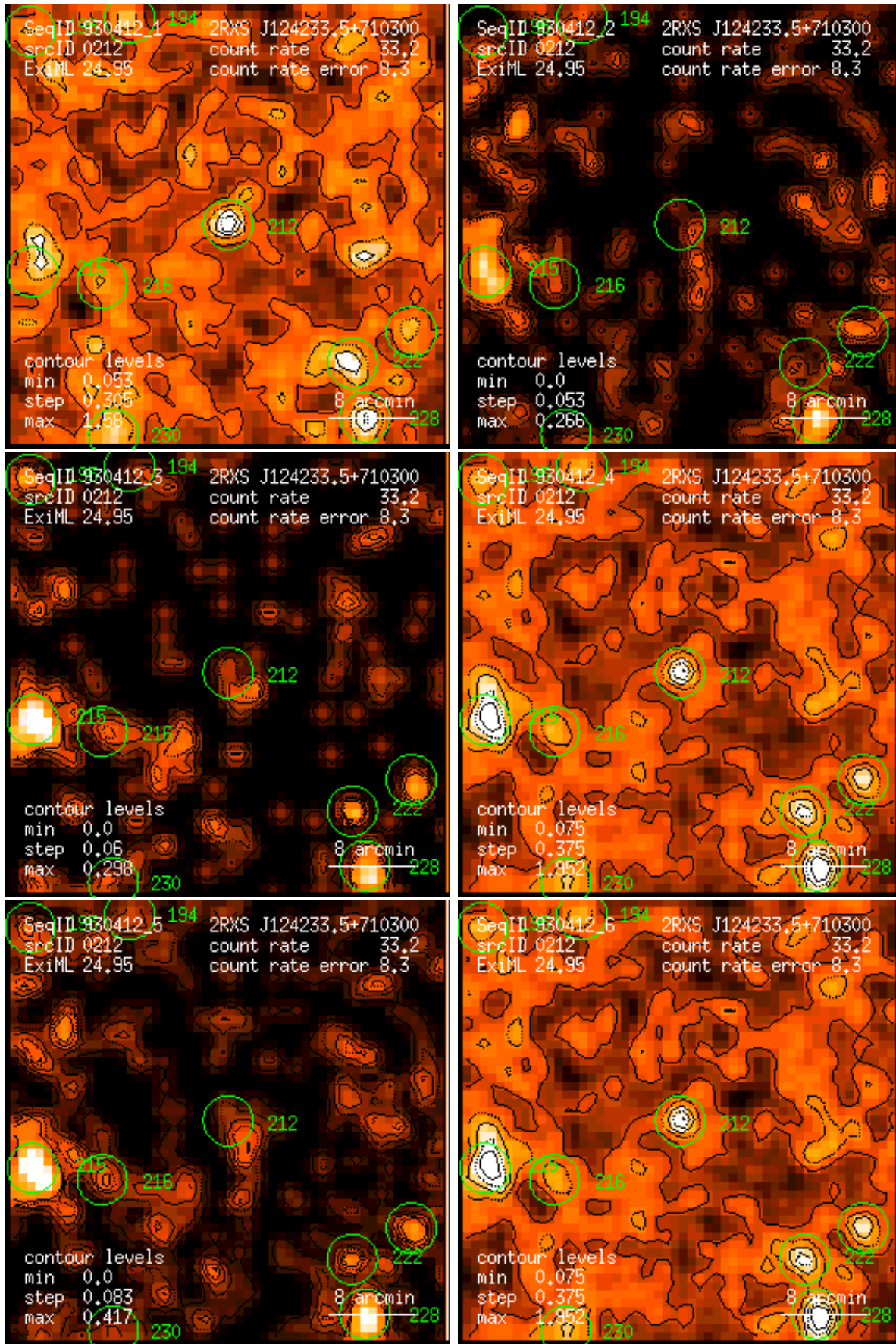
Figure 212: RASS 930412: detection 0212: band rate images, Gaussian filter: (1) PSPC channels 11 – 41, (2) 52 – 90, (3) 91 – 201, (4) 11 – 235, (5) 52 – 201, (6) 11 – 201. Broad band rates in counts/ks. Band rate contour levels in counts/ks/arcmin 2 .
