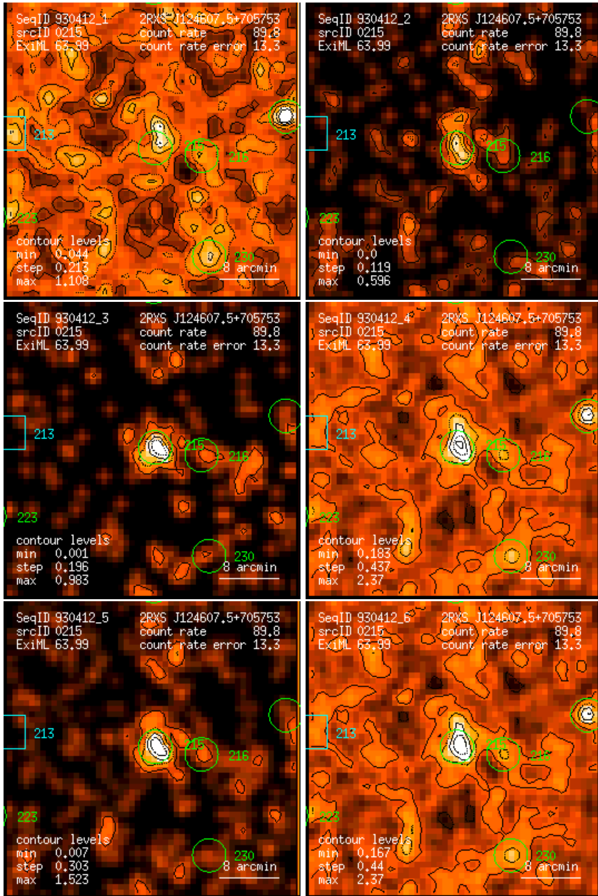
Figure 215: RASS 930412: detection 0215: band rate images, Gaussian filter: (1) PSPC channels 11 – 41, (2) 52 – 90, (3) 91 – 201, (4) 11 – 235, (5) 52 – 201, (6) 11 – 201. Broad band rates in counts/ks. Band rate contour levels in counts/ks/arcmin 2 .
