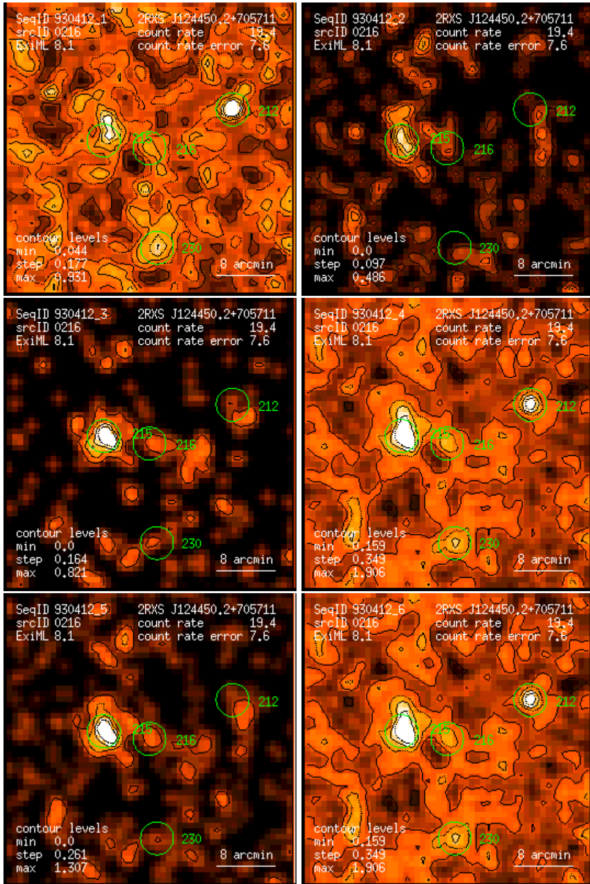
Figure 216: RASS 930412: detection 0216: band rate images, Gaussian filter: (1) PSPC channels 11 – 41, (2) 52 – 90, (3) 91 – 201, (4) 11 – 235, (5) 52 – 201, (6) 11 – 201. Broad band rates in counts/ks. Band rate contour levels in counts/ks/arcmin 2 .
