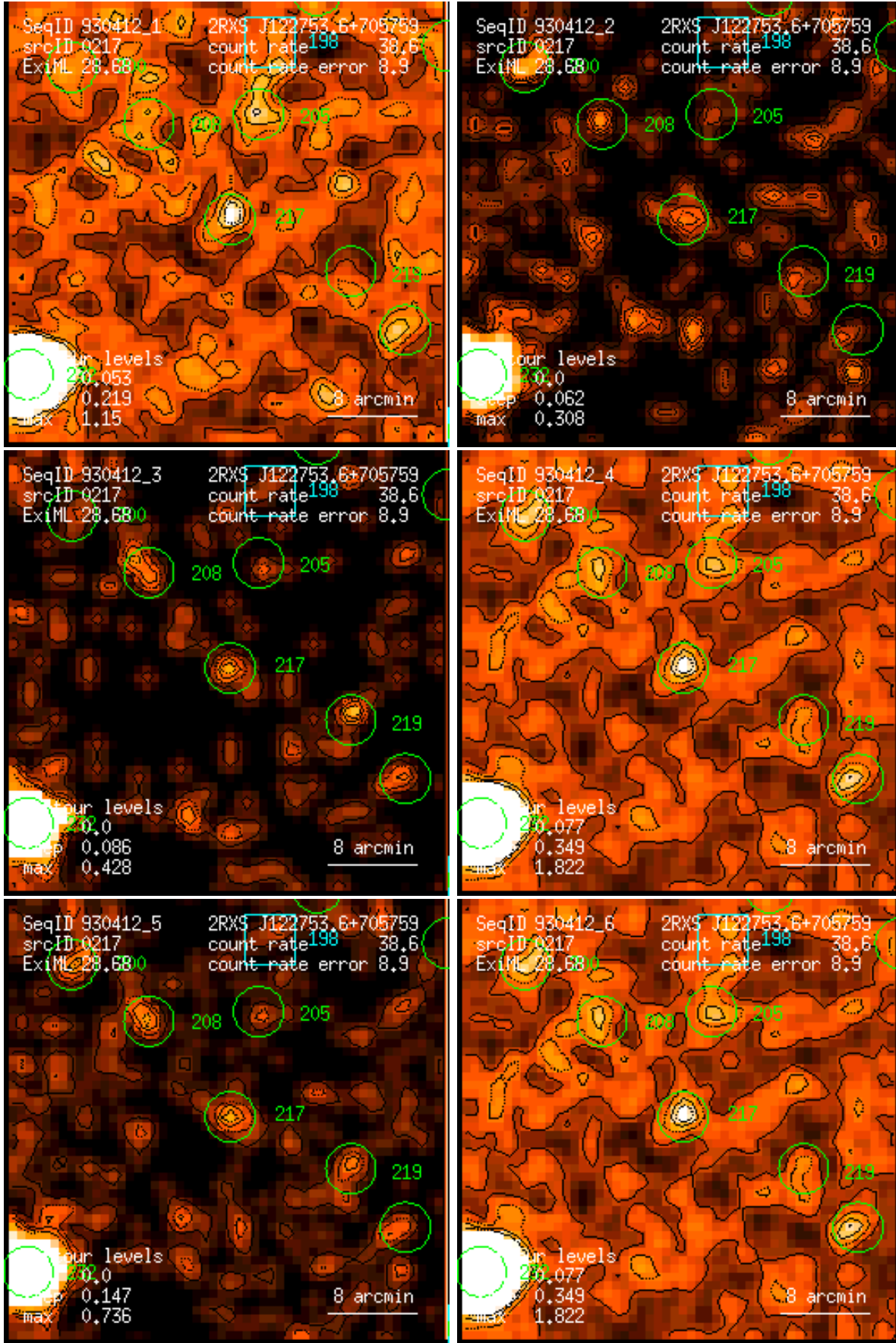
Figure 217: RASS 930412: detection 0217: band rate images, Gaussian filter: (1) PSPC channels 11 – 41, (2) 52 – 90, (3) 91 – 201, (4) 11 – 235, (5) 52 – 201, (6) 11 – 201. Broad band rates in counts/ks. Band rate contour levels in counts/ks/arcmin 2 .
