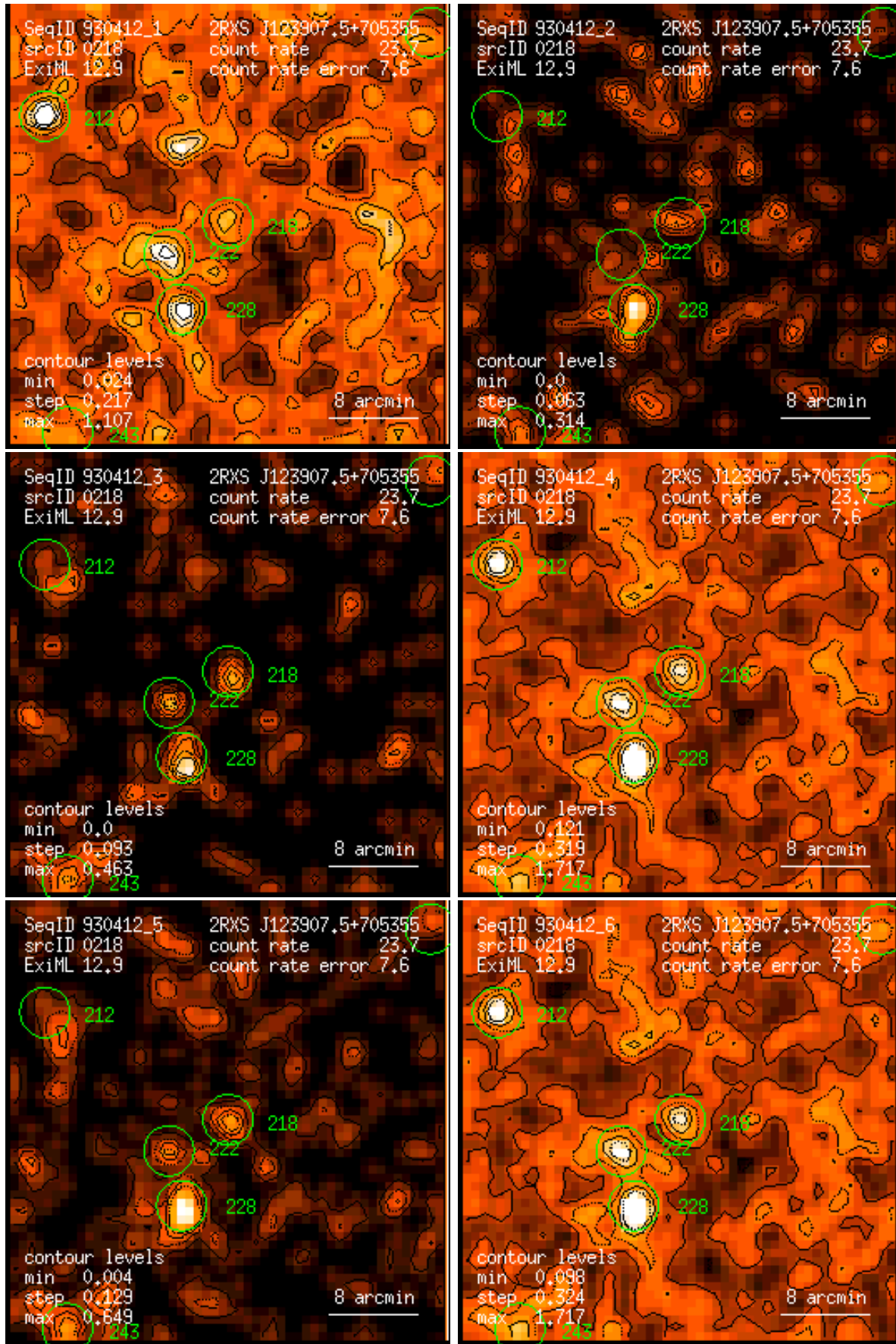
Figure 218: RASS 930412: detection 0218: band rate images, Gaussian filter: (1) PSPC channels 11 – 41, (2) 52 – 90, (3) 91 – 201, (4) 11 – 235, (5) 52 – 201, (6) 11 – 201. Broad band rates in counts/ks. Band rate contour levels in counts/ks/arcmin 2 .
