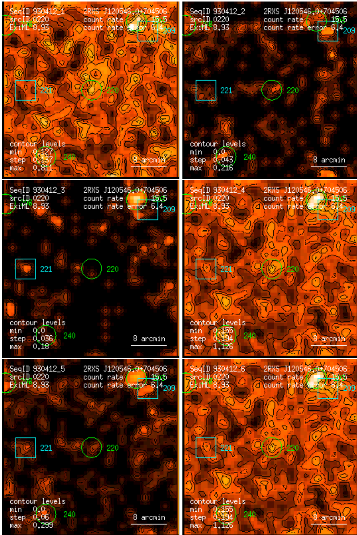
Figure 220: RASS 930412: detection 0220: band rate images, Gaussian filter: (1) PSPC channels 11 – 41, (2) 52 – 90, (3) 91 – 201, (4) 11 – 235, (5) 52 – 201, (6) 11 – 201. Broad band rates in counts/ks. Band rate contour levels in counts/ks/arcmin 2 .
