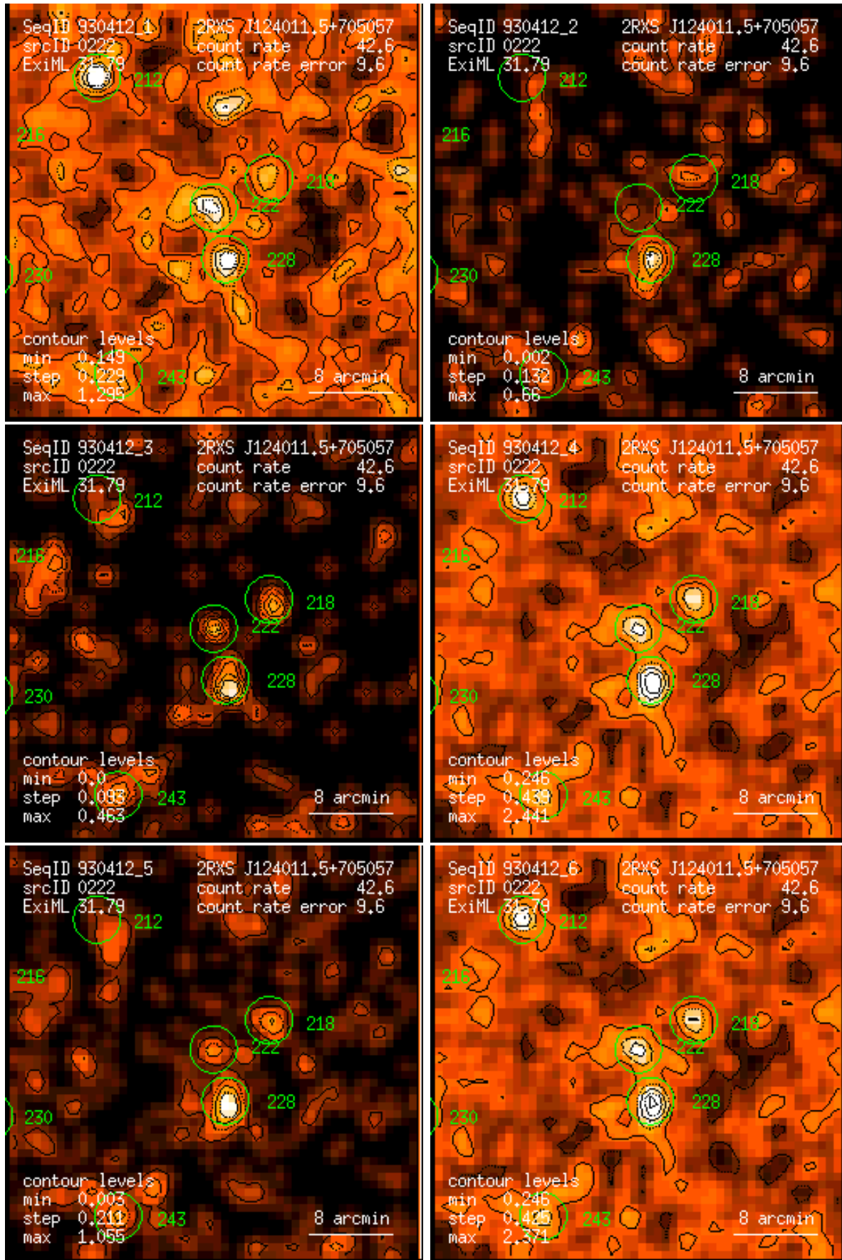
Figure 222: RASS 930412: detection 0222: band rate images, Gaussian filter: (1) PSPC channels 11 – 41, (2) 52 – 90, (3) 91 – 201, (4) 11 – 235, (5) 52 – 201, (6) 11 – 201. Broad band rates in counts/ks. Band rate contour levels in counts/ks/arcmin 2 .
