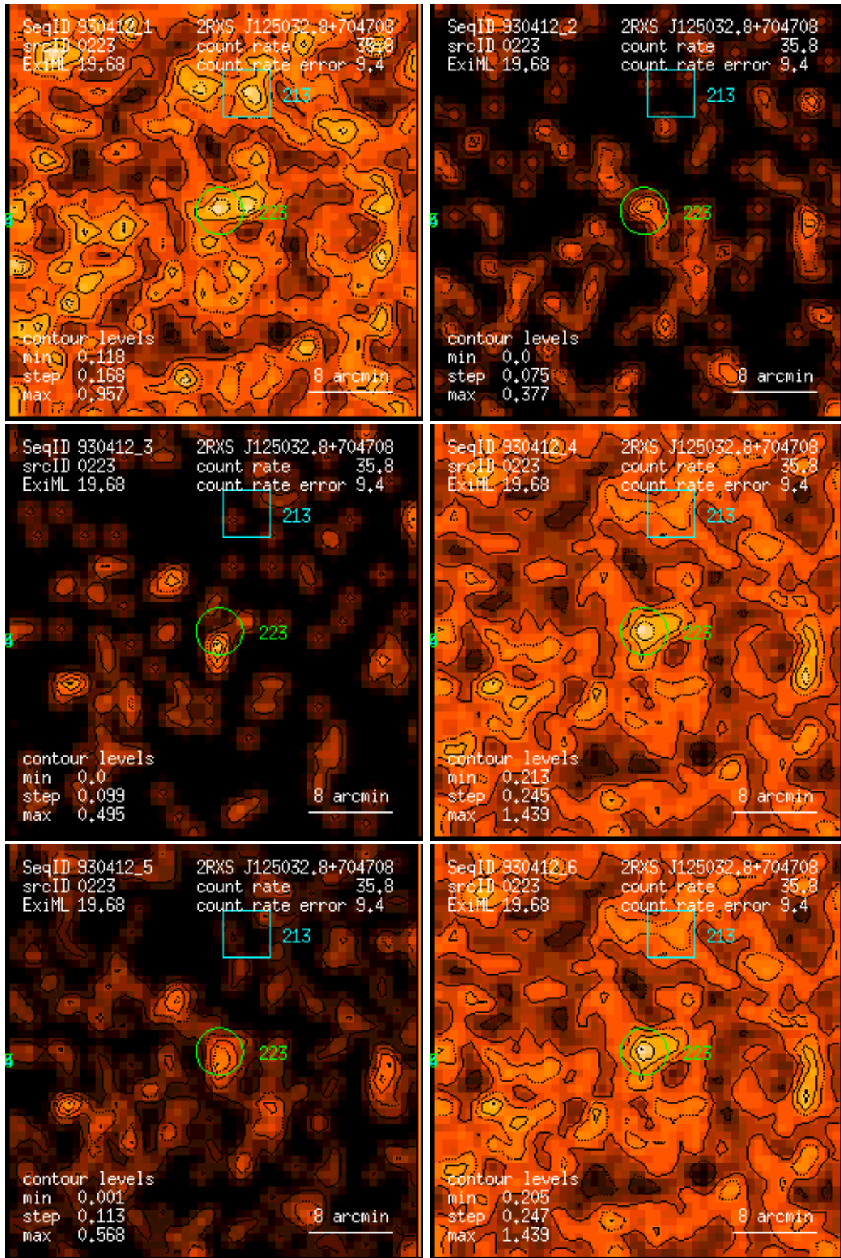
Figure 223: RASS 930412: detection 0223: band rate images, Gaussian filter: (1) PSPC channels 11 – 41, (2) 52 – 90, (3) 91 – 201, (4) 11 – 235, (5) 52 – 201, (6) 11 – 201. Broad band rates in counts/ks. Band rate contour levels in counts/ks/arcmin 2 .
