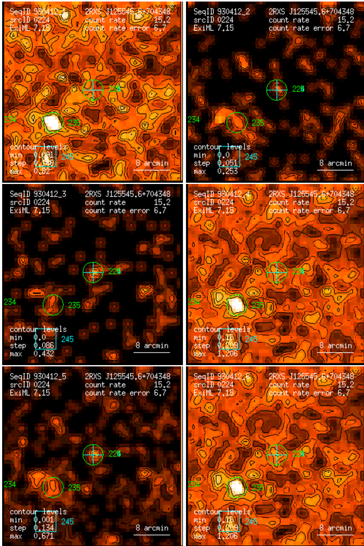
Figure 224: RASS 930412: detection 0224: band rate images, Gaussian filter: (1) PSPC channels 11 – 41, (2) 52 – 90, (3) 91 – 201, (4) 11 – 235, (5) 52 – 201, (6) 11 – 201. Broad band rates in counts/ks. Band rate contour levels in counts/ks/arcmin 2 .
