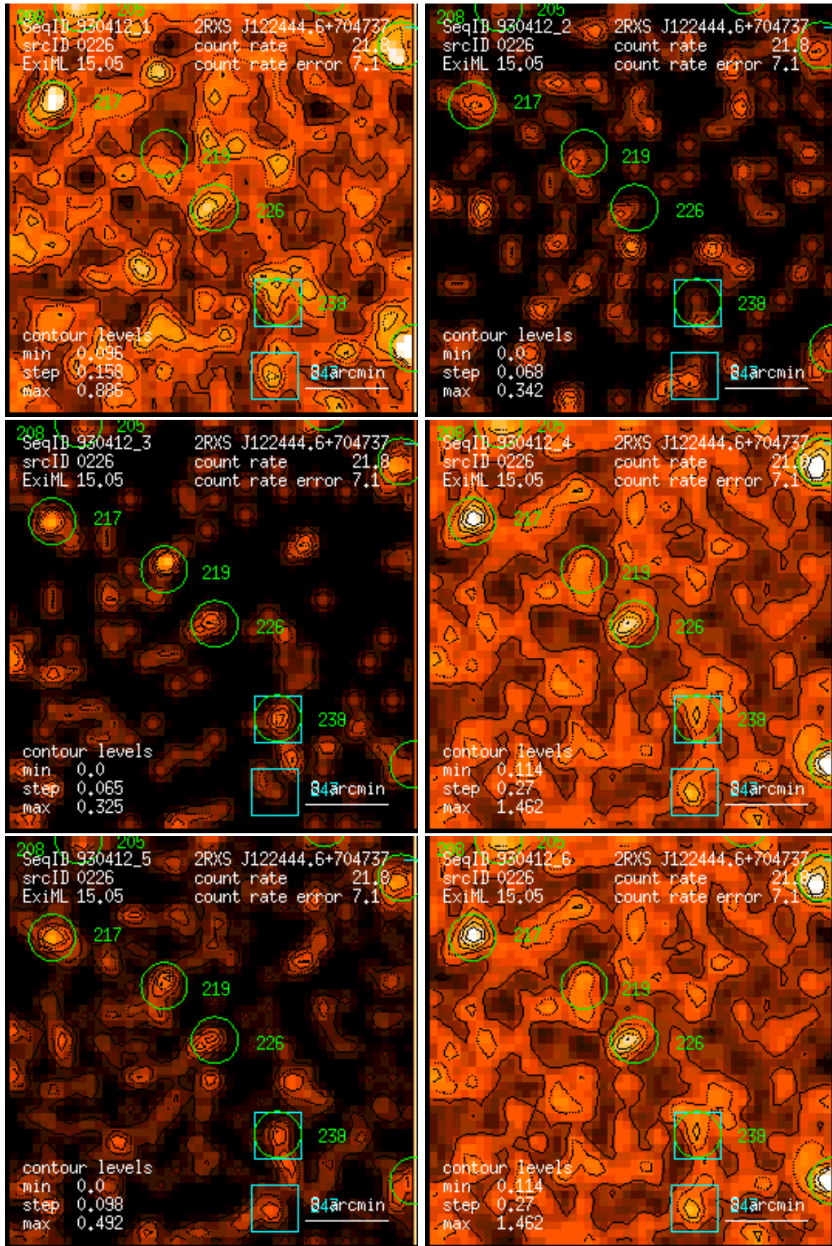
Figure 226: RASS 930412: detection 0226: band rate images, Gaussian filter: (1) PSPC channels 11 – 41, (2) 52 – 90, (3) 91 – 201, (4) 11 – 235, (5) 52 – 201, (6) 11 – 201. Broad band rates in counts/ks. Band rate contour levels in counts/ks/arcmin 2 .
