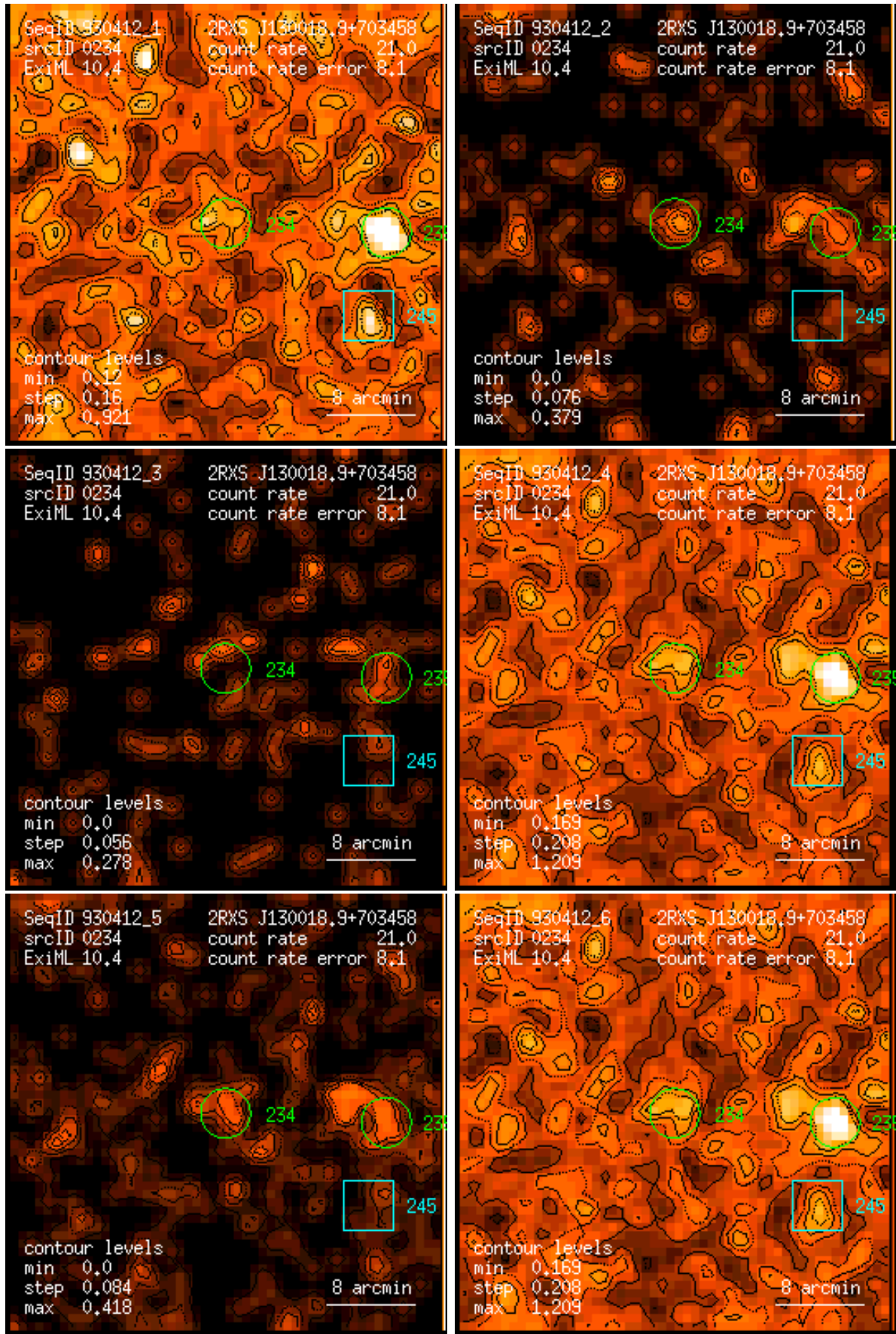
Figure 234: RASS 930412: detection 0234: band rate images, Gaussian filter: (1) PSPC channels 11 – 41, (2) 52 – 90, (3) 91 – 201, (4) 11 – 235, (5) 52 – 201, (6) 11 – 201. Broad band rates in counts/ks. Band rate contour levels in counts/ks/arcmin 2 .
