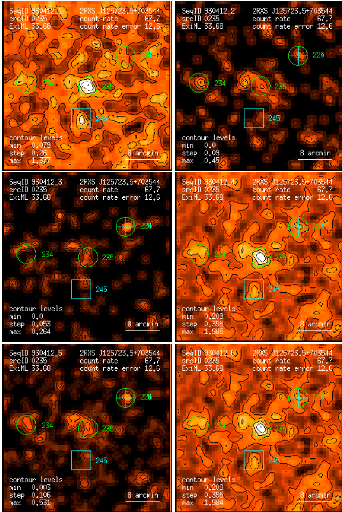
Figure 235: RASS 930412: detection 0235: band rate images, Gaussian filter: (1) PSPC channels 11 – 41, (2) 52 – 90, (3) 91 – 201, (4) 11 – 235, (5) 52 – 201, (6) 11 – 201. Broad band rates in counts/ks. Band rate contour levels in counts/ks/arcmin 2 .
