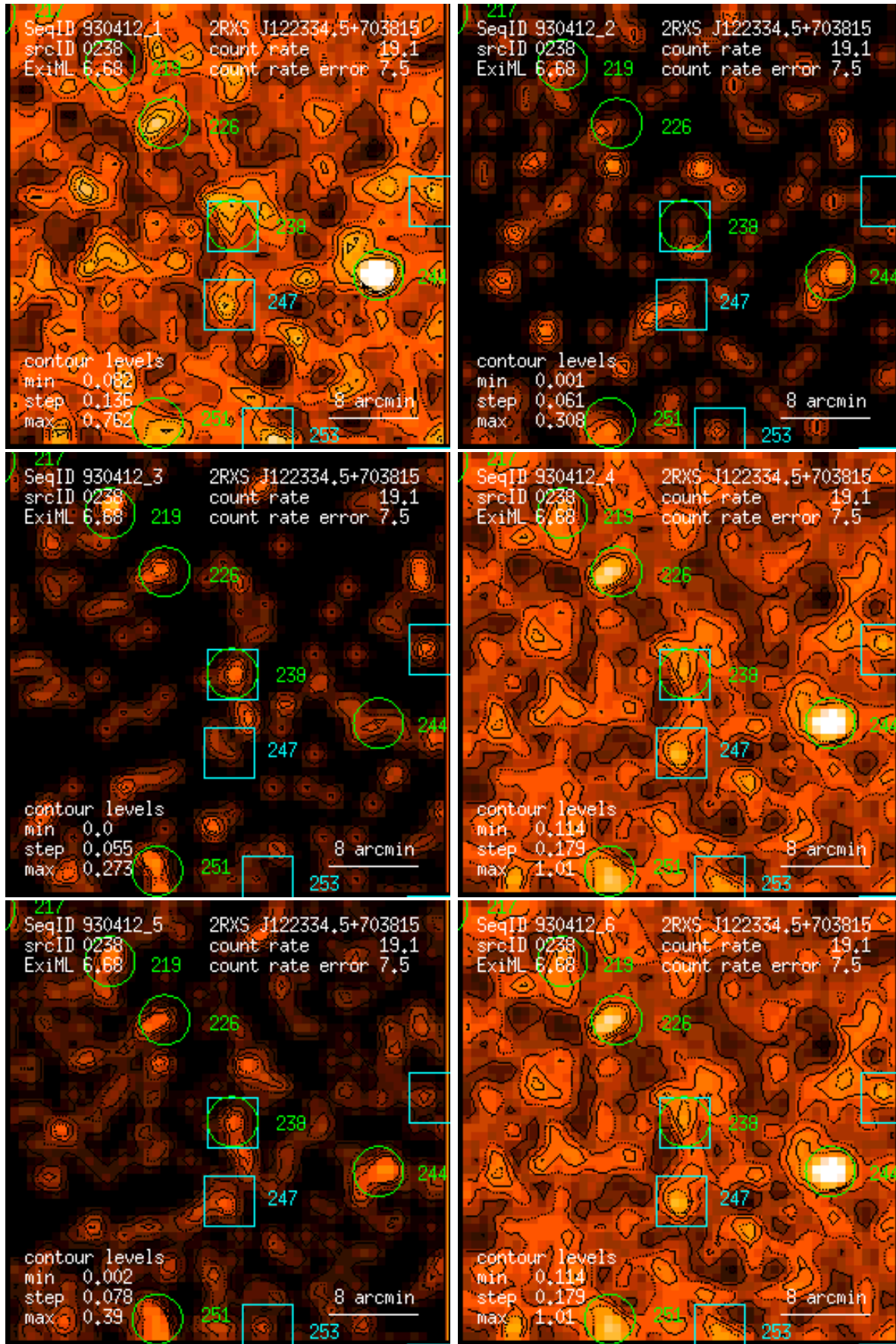
Figure 238: RASS 930412: detection 0238: band rate images, Gaussian filter: (1) PSPC channels 11 – 41, (2) 52 – 90, (3) 91 – 201, (4) 11 – 235, (5) 52 – 201, (6) 11 – 201. Broad band rates in counts/ks. Band rate contour levels in counts/ks/arcmin 2 .
