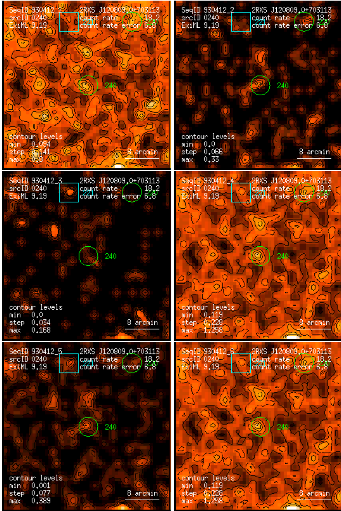
Figure 240: RASS 930412: detection 0240: band rate images, Gaussian filter: (1) PSPC channels 11 – 41, (2) 52 – 90, (3) 91 – 201, (4) 11 – 235, (5) 52 – 201, (6) 11 – 201. Broad band rates in counts/ks. Band rate contour levels in counts/ks/arcmin 2 .
