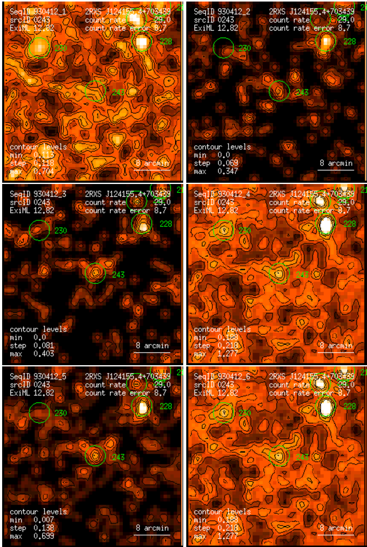
Figure 243: RASS 930412: detection 0243: band rate images, Gaussian filter: (1) PSPC channels 11 – 41, (2) 52 – 90, (3) 91 – 201, (4) 11 – 235, (5) 52 – 201, (6) 11 – 201. Broad band rates in counts/ks. Band rate contour levels in counts/ks/arcmin 2 .
