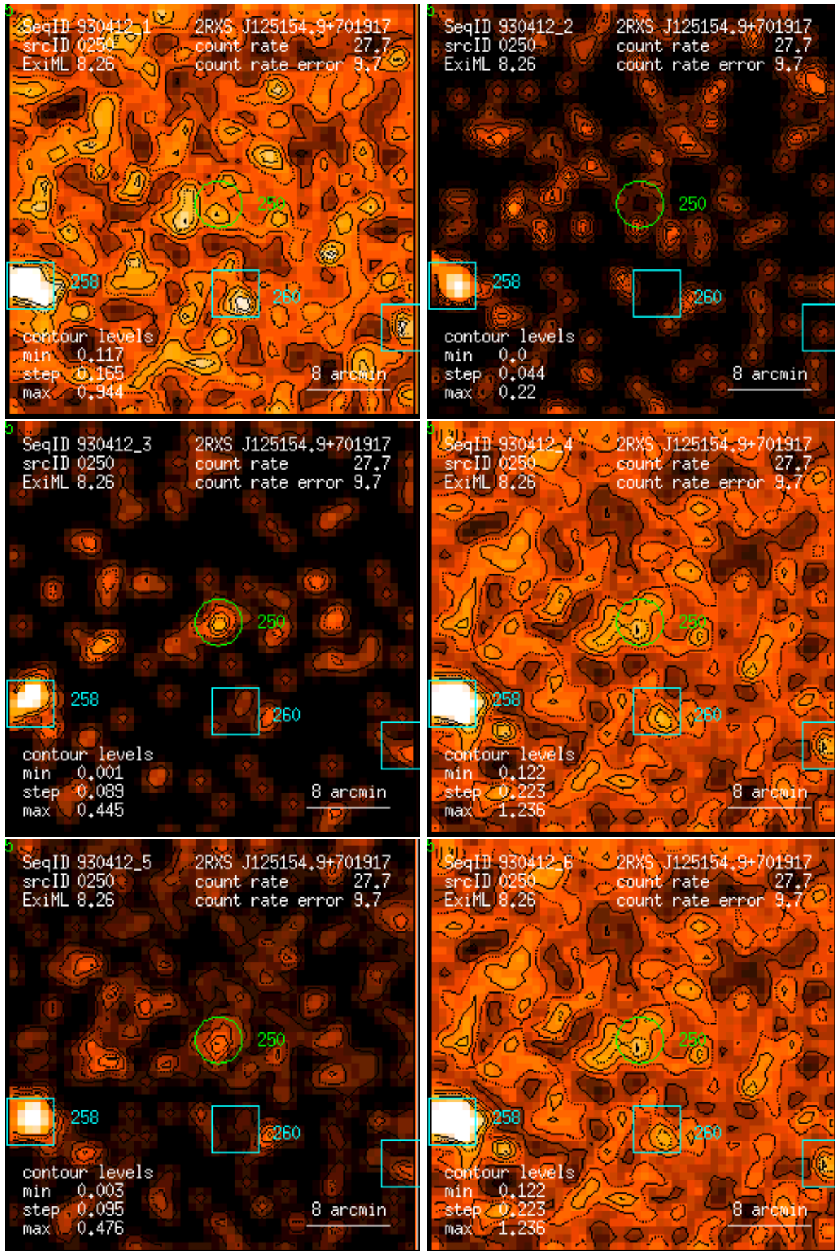
Figure 250: RASS 930412: detection 0250: band rate images, Gaussian filter: (1) PSPC channels 11 – 41, (2) 52 – 90, (3) 91 – 201, (4) 11 – 235, (5) 52 – 201, (6) 11 – 201. Broad band rates in counts/ks. Band rate contour levels in counts/ks/arcmin 2 .
