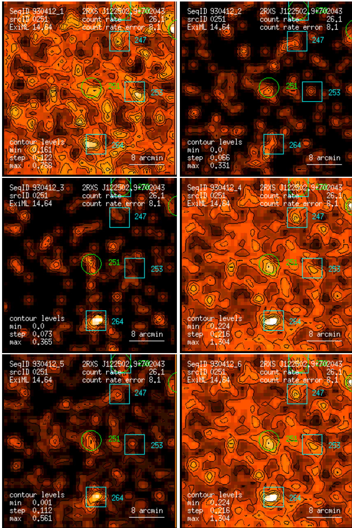
Figure 251: RASS 930412: detection 0251: band rate images, Gaussian filter: (1) PSPC channels 11 – 41, (2) 52 – 90, (3) 91 – 201, (4) 11 – 235, (5) 52 – 201, (6) 11 – 201. Broad band rates in counts/ks. Band rate contour levels in counts/ks/arcmin 2 .
