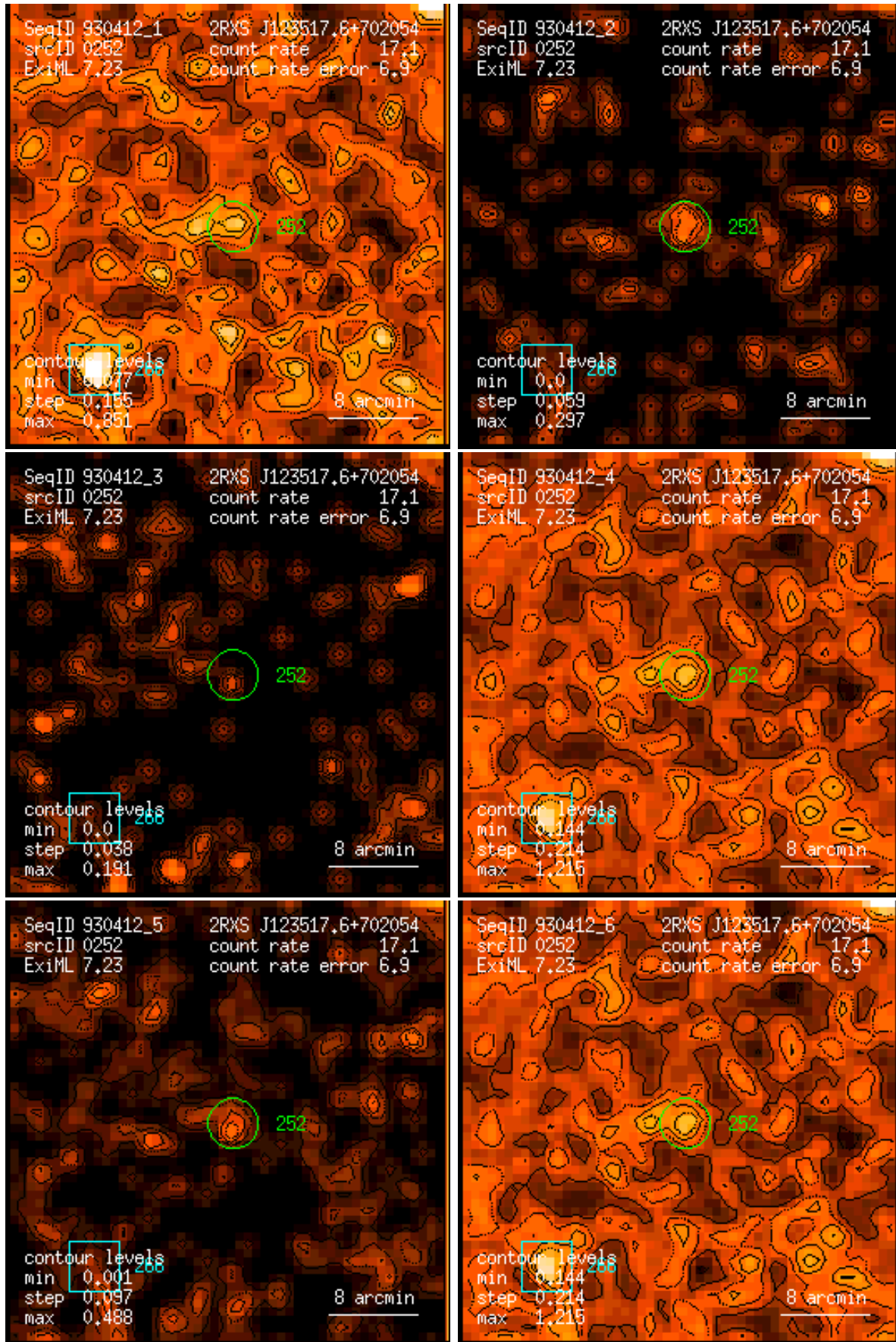
Figure 252: RASS 930412: detection 0252: band rate images, Gaussian filter: (1) PSPC channels 11 – 41, (2) 52 – 90, (3) 91 – 201, (4) 11 – 235, (5) 52 – 201, (6) 11 – 201. Broad band rates in counts/ks. Band rate contour levels in counts/ks/arcmin 2 .
