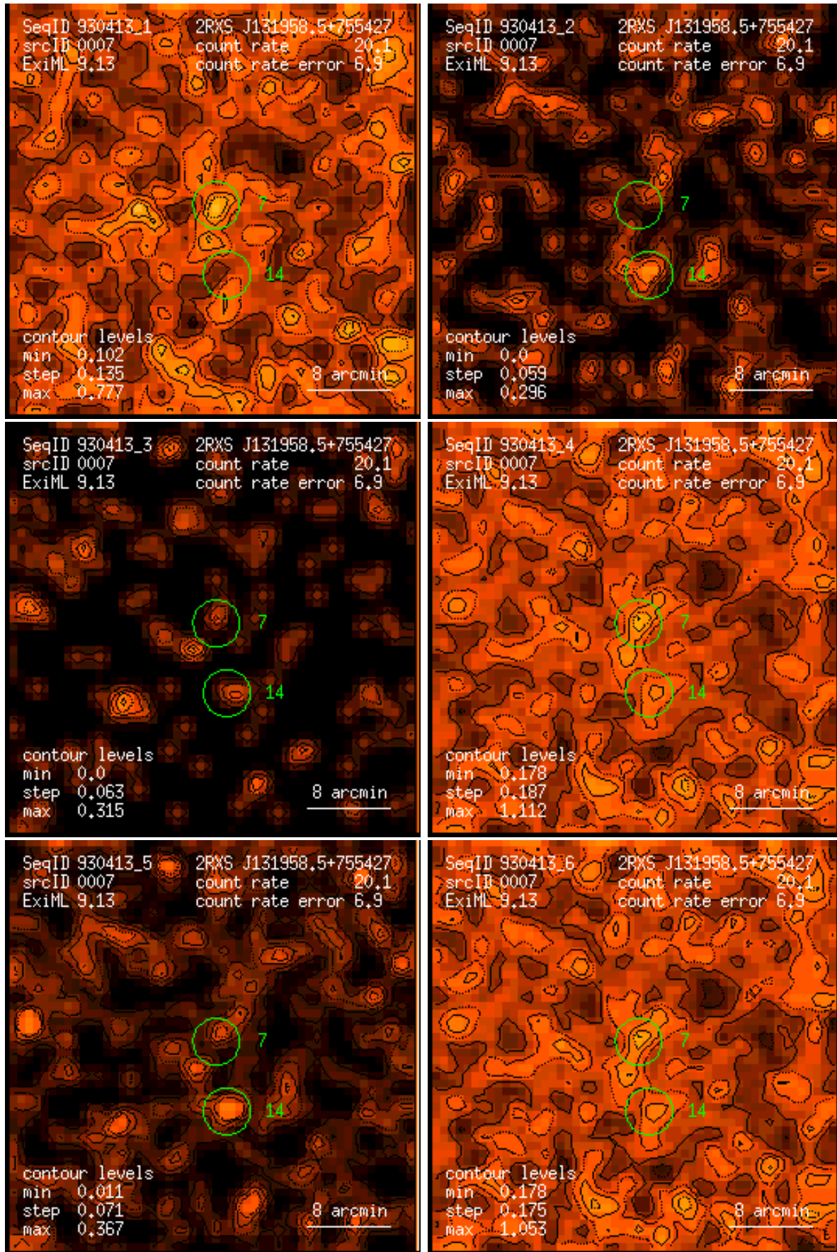
Figure 7: RASS 930413: detection 0007: band rate images, Gaussian filter: (1) PSPC channels 11 – 41, (2) 52 – 90, (3) 91 – 201, (4) 11 – 235, (5) 52 – 201, (6) 11 – 201. Broad band rates in counts/ks. Band rate contour levels in counts/ks/arcmin 2 .
