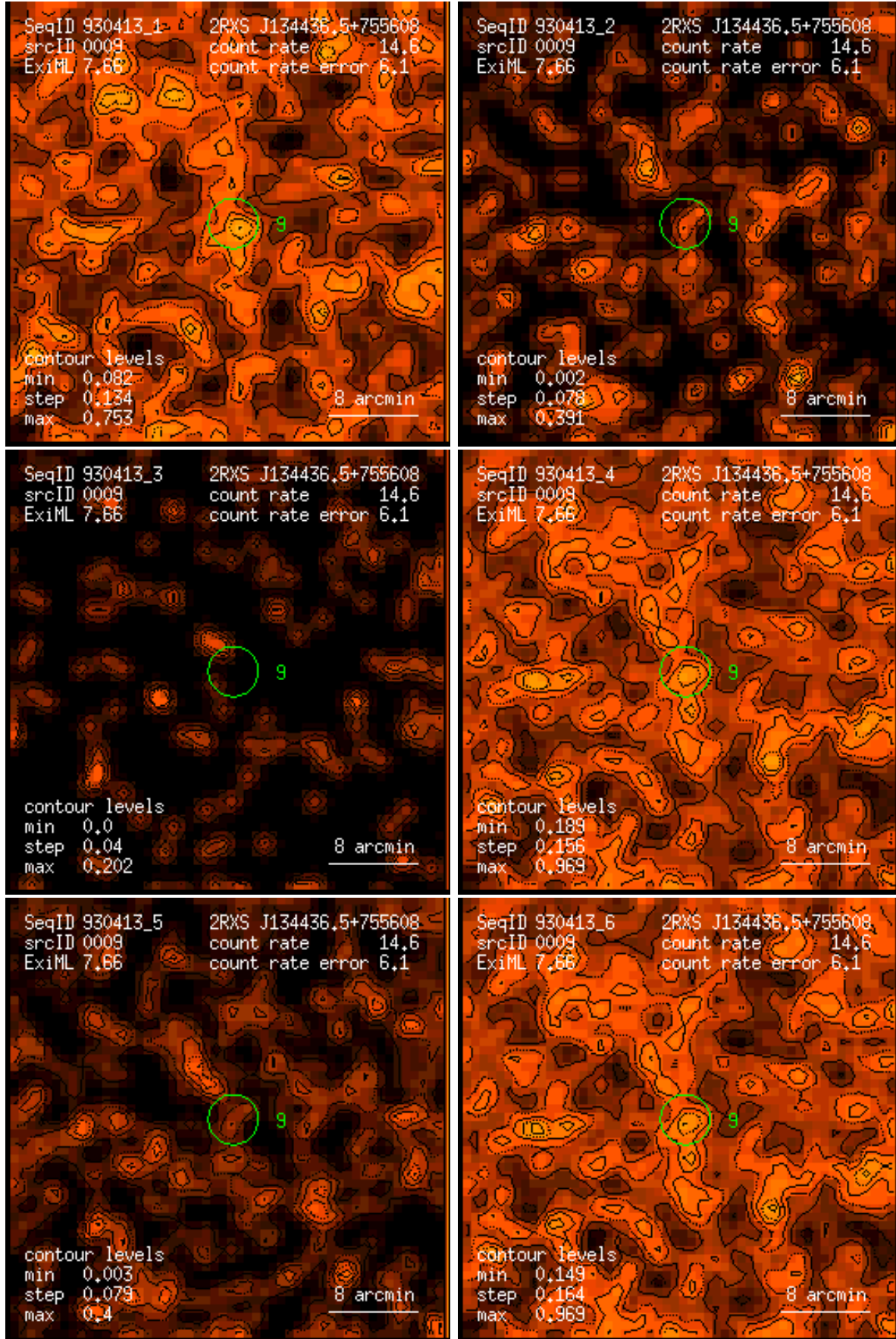
Figure 9: RASS 930413: detection 0009: band rate images, Gaussian filter: (1) PSPC channels 11 – 41, (2) 52 – 90, (3) 91 – 201, (4) 11 – 235, (5) 52 – 201, (6) 11 – 201. Broad band rates in counts/ks. Band rate contour levels in counts/ks/arcmin 2 .
