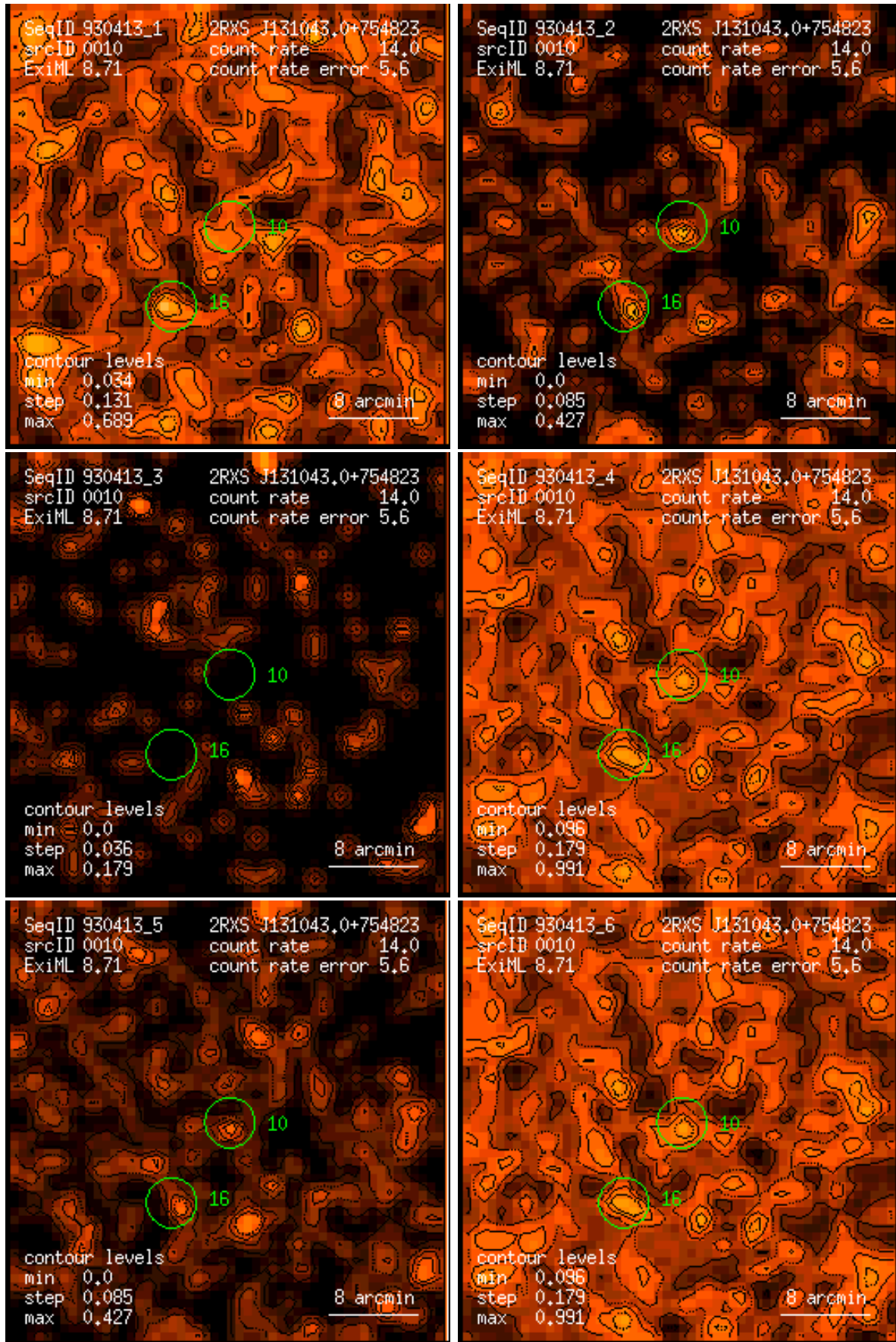
Figure 10: RASS 930413: detection 0010: band rate images, Gaussian filter: (1) PSPC channels 11 – 41, (2) 52 – 90, (3) 91 – 201, (4) 11 – 235, (5) 52 – 201, (6) 11 – 201. Broad band rates in counts/ks. Band rate contour levels in counts/ks/arcmin 2 .
