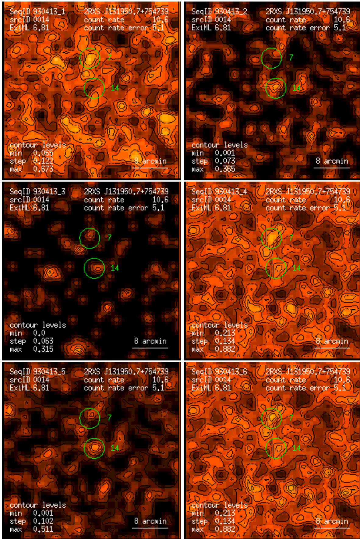
Figure 14: RASS 930413: detection 0014: band rate images, Gaussian filter: (1) PSPC channels 11 – 41, (2) 52 – 90, (3) 91 – 201, (4) 11 – 235, (5) 52 – 201, (6) 11 – 201. Broad band rates in counts/ks. Band rate contour levels in counts/ks/arcmin 2 .
