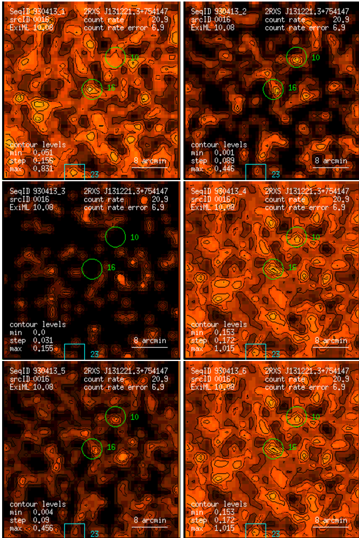
Figure 16: RASS 930413: detection 0016: band rate images, Gaussian filter: (1) PSPC channels 11 – 41, (2) 52 – 90, (3) 91 – 201, (4) 11 – 235, (5) 52 – 201, (6) 11 – 201. Broad band rates in counts/ks. Band rate contour levels in counts/ks/arcmin 2 .
