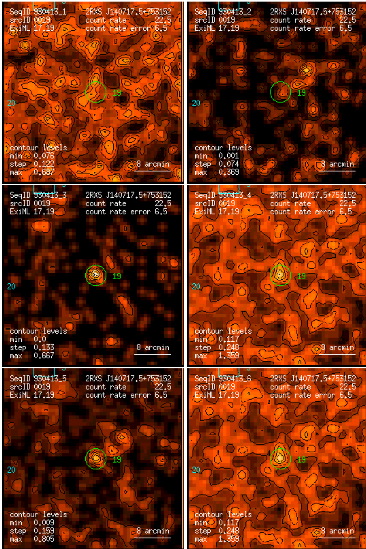
Figure 19: RASS 930413: detection 0019: band rate images, Gaussian filter: (1) PSPC channels 11 – 41, (2) 52 – 90, (3) 91 – 201, (4) 11 – 235, (5) 52 – 201, (6) 11 – 201. Broad band rates in counts/ks. Band rate contour levels in counts/ks/arcmin 2 .
