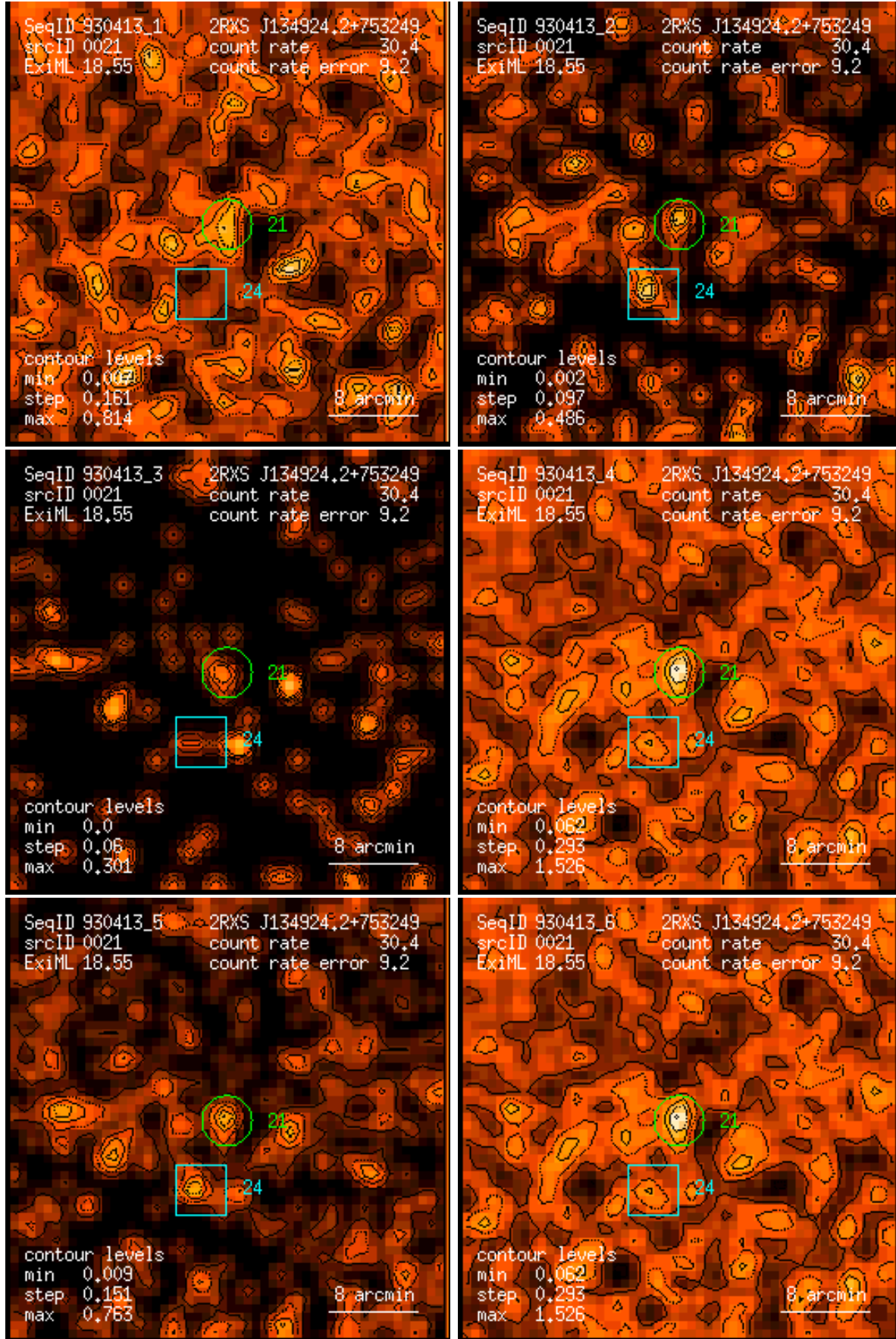
Figure 21: RASS 930413: detection 0021: band rate images, Gaussian filter: (1) PSPC channels 11 – 41, (2) 52 – 90, (3) 91 – 201, (4) 11 – 235, (5) 52 – 201, (6) 11 – 201. Broad band rates in counts/ks. Band rate contour levels in counts/ks/arcmin 2 .
