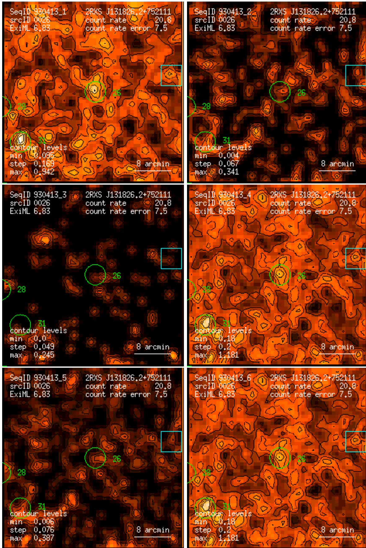
Figure 26: RASS 930413: detection 0026: band rate images, Gaussian filter: (1) PSPC channels 11 – 41, (2) 52 – 90, (3) 91 – 201, (4) 11 – 235, (5) 52 – 201, (6) 11 – 201. Broad band rates in counts/ks. Band rate contour levels in counts/ks/arcmin 2 .
