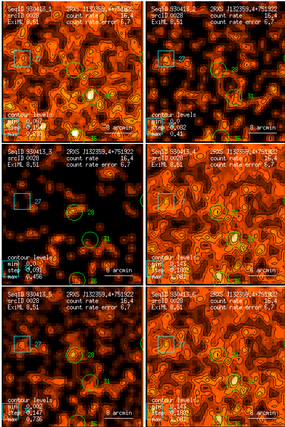
Figure 28: RASS 930413: detection 0028: band rate images, Gaussian filter: (1) PSPC channels 11 – 41, (2) 52 – 90, (3) 91 – 201, (4) 11 – 235, (5) 52 – 201, (6) 11 – 201. Broad band rates in counts/ks. Band rate contour levels in counts/ks/arcmin 2 .
