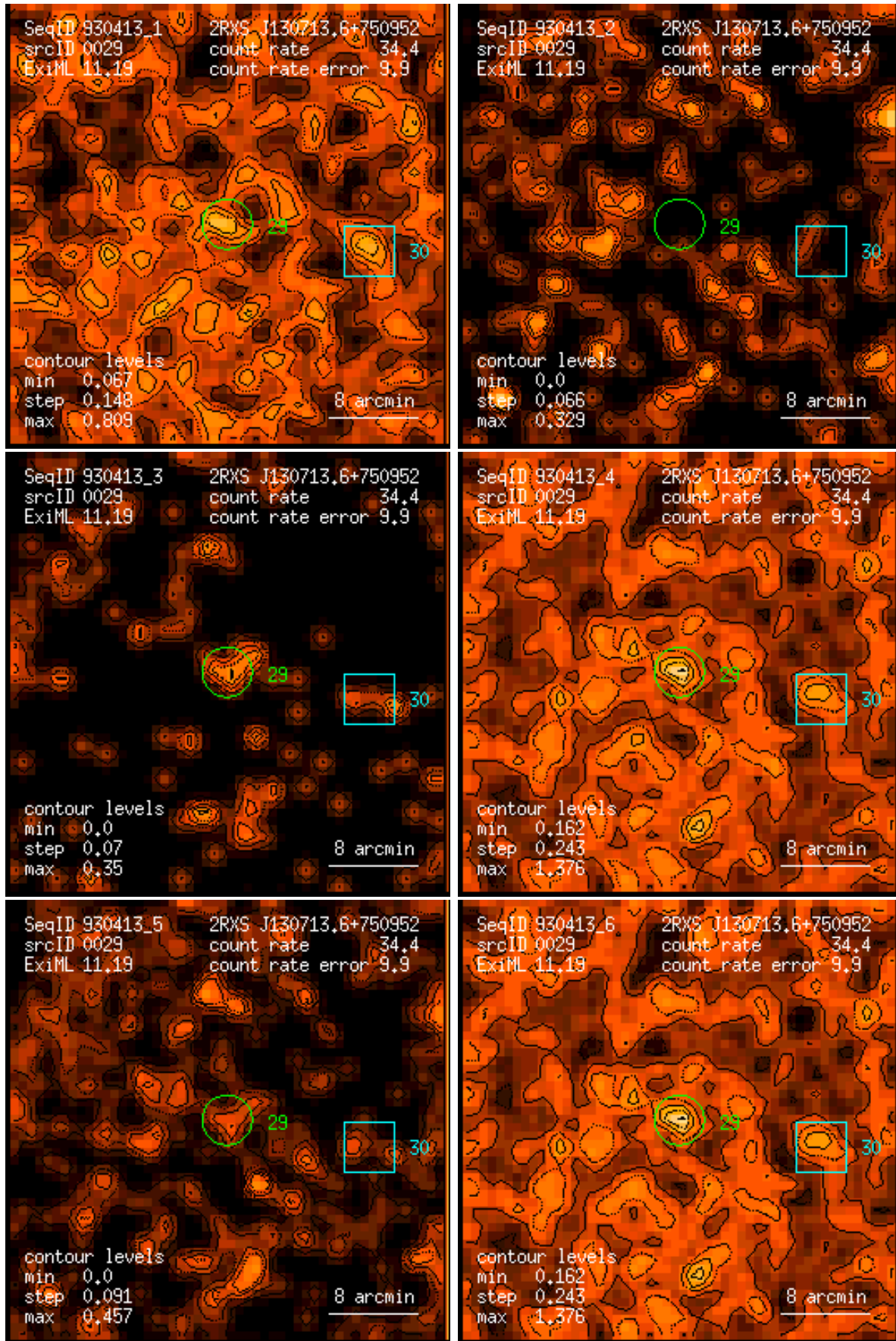
Figure 29: RASS 930413: detection 0029: band rate images, Gaussian filter: (1) PSPC channels 11 – 41, (2) 52 – 90, (3) 91 – 201, (4) 11 – 235, (5) 52 – 201, (6) 11 – 201. Broad band rates in counts/ks. Band rate contour levels in counts/ks/arcmin 2 .
