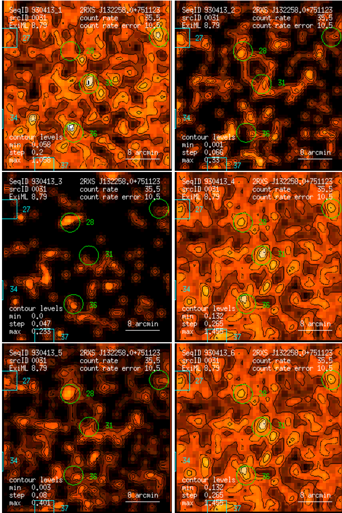
Figure 31: RASS 930413: detection 0031: band rate images, Gaussian filter: (1) PSPC channels 11 – 41, (2) 52 – 90, (3) 91 – 201, (4) 11 – 235, (5) 52 – 201, (6) 11 – 201. Broad band rates in counts/ks. Band rate contour levels in counts/ks/arcmin 2 .
