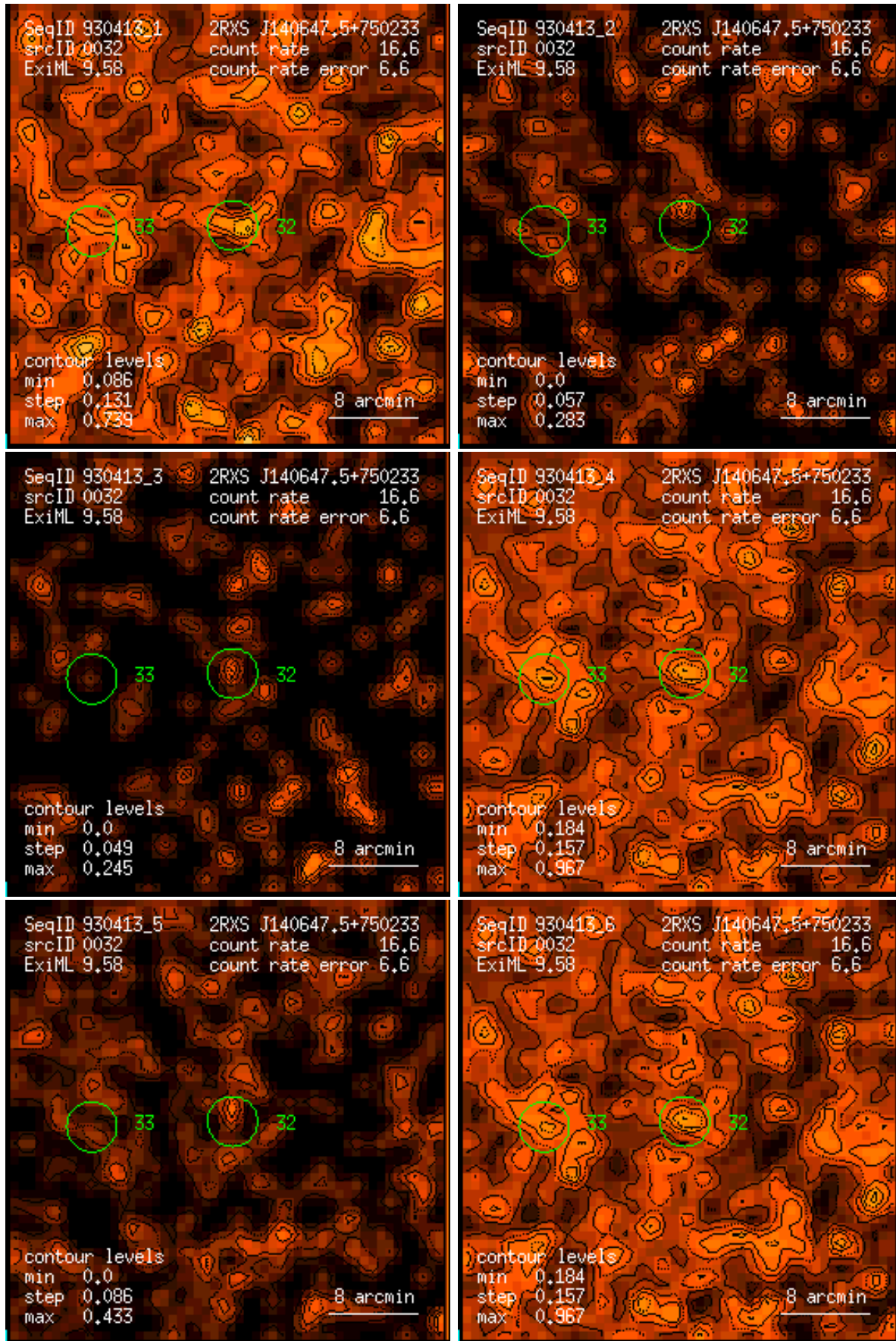
Figure 32: RASS 930413: detection 0032: band rate images, Gaussian filter: (1) PSPC channels 11 – 41, (2) 52 – 90, (3) 91 – 201, (4) 11 – 235, (5) 52 – 201, (6) 11 – 201. Broad band rates in counts/ks. Band rate contour levels in counts/ks/arcmin 2 .
