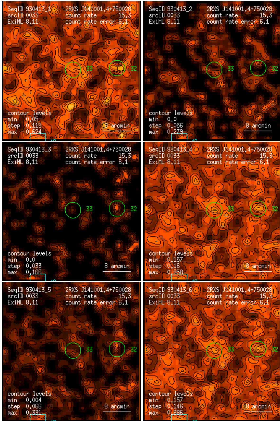
Figure 33: RASS 930413: detection 0033: band rate images, Gaussian filter: (1) PSPC channels 11 – 41, (2) 52 – 90, (3) 91 – 201, (4) 11 – 235, (5) 52 – 201, (6) 11 – 201. Broad band rates in counts/ks. Band rate contour levels in counts/ks/arcmin 2 .
