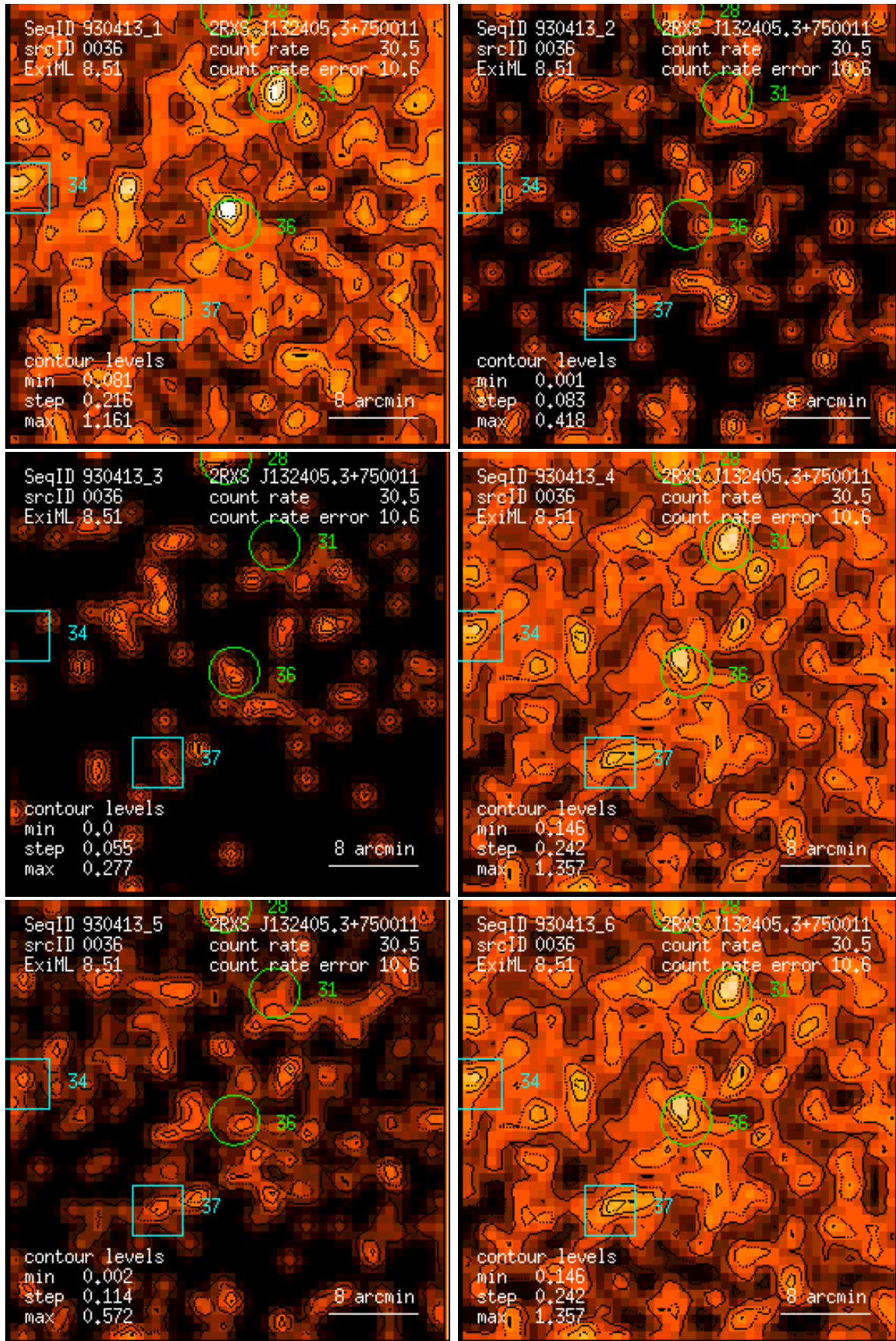
Figure 36: RASS 930413: detection 0036: band rate images, Gaussian filter: (1) PSPC channels 11 – 41, (2) 52 – 90, (3) 91 – 201, (4) 11 – 235, (5) 52 – 201, (6) 11 – 201. Broad band rates in counts/ks. Band rate contour levels in counts/ks/arcmin 2 .
