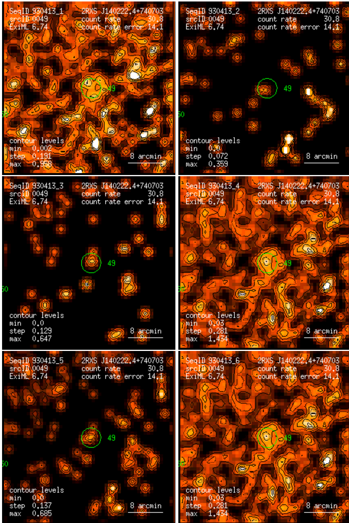
Figure 49: RASS 930413: detection 0049: band rate images, Gaussian filter: (1) PSPC channels 11 – 41, (2) 52 – 90, (3) 91 – 201, (4) 11 – 235, (5) 52 – 201, (6) 11 – 201. Broad band rates in counts/ks. Band rate contour levels in counts/ks/arcmin 2 .
