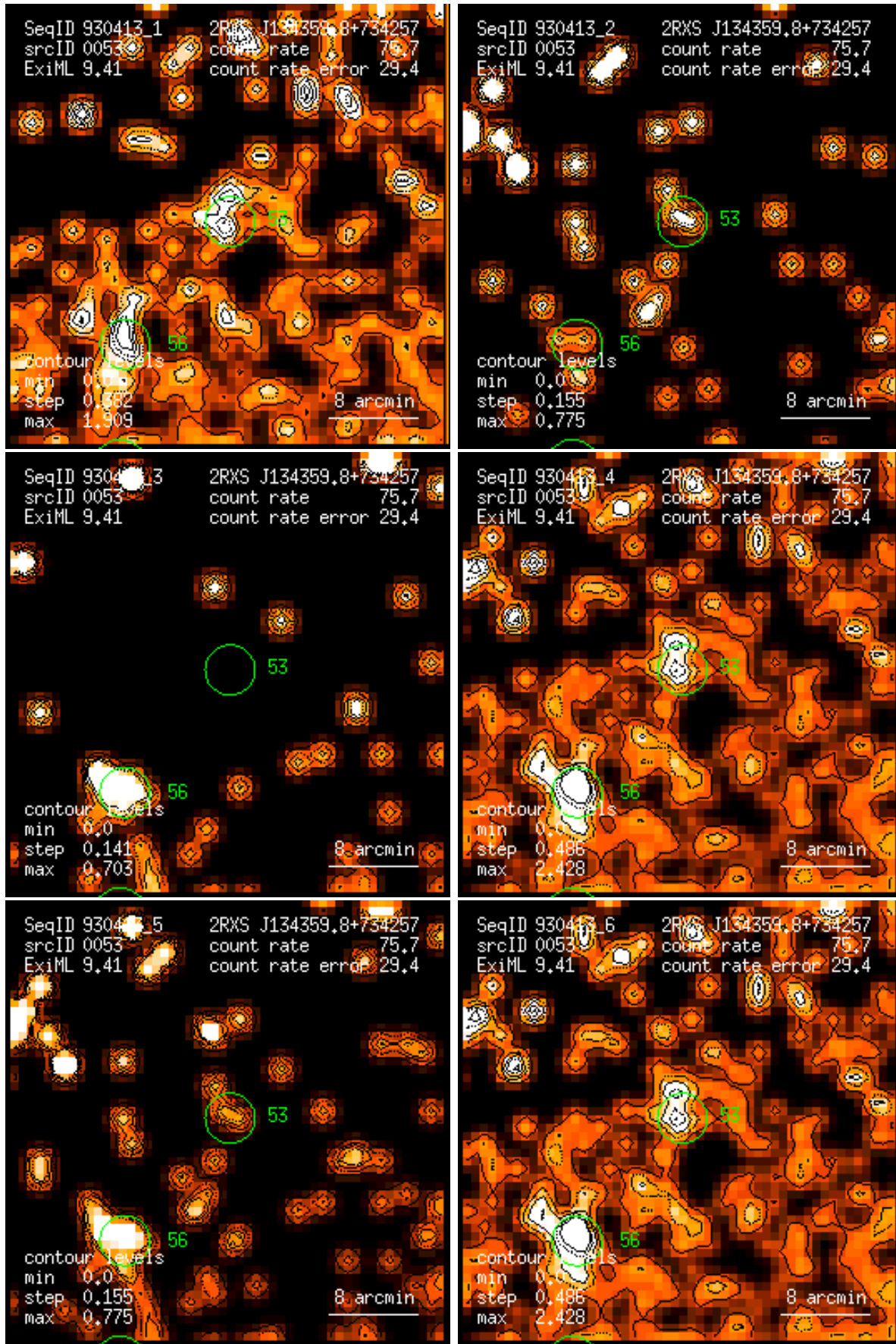
Figure 53: RASS 930413: detection 0053: band rate images, Gaussian filter: (1) PSPC channels 11 – 41, (2) 52 – 90, (3) 91 – 201, (4) 11 – 235, (5) 52 – 201, (6) 11 – 201. Broad band rates in counts/ks. Band rate contour levels in counts/ks/arcmin 2 .
