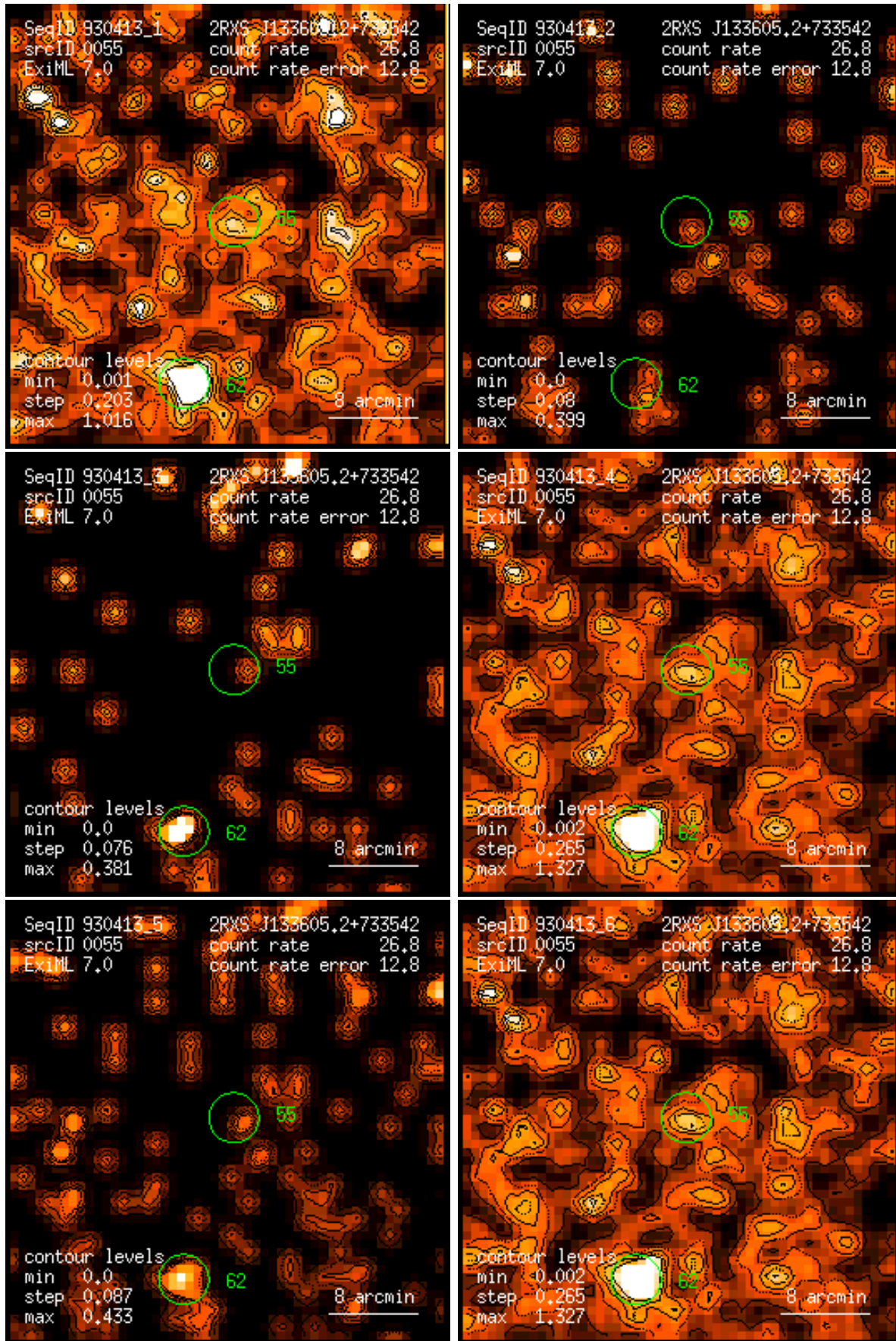
Figure 55: RASS 930413: detection 0055: band rate images, Gaussian filter: (1) PSPC channels 11 – 41, (2) 52 – 90, (3) 91 – 201, (4) 11 – 235, (5) 52 – 201, (6) 11 – 201. Broad band rates in counts/ks. Band rate contour levels in counts/ks/arcmin 2 .
