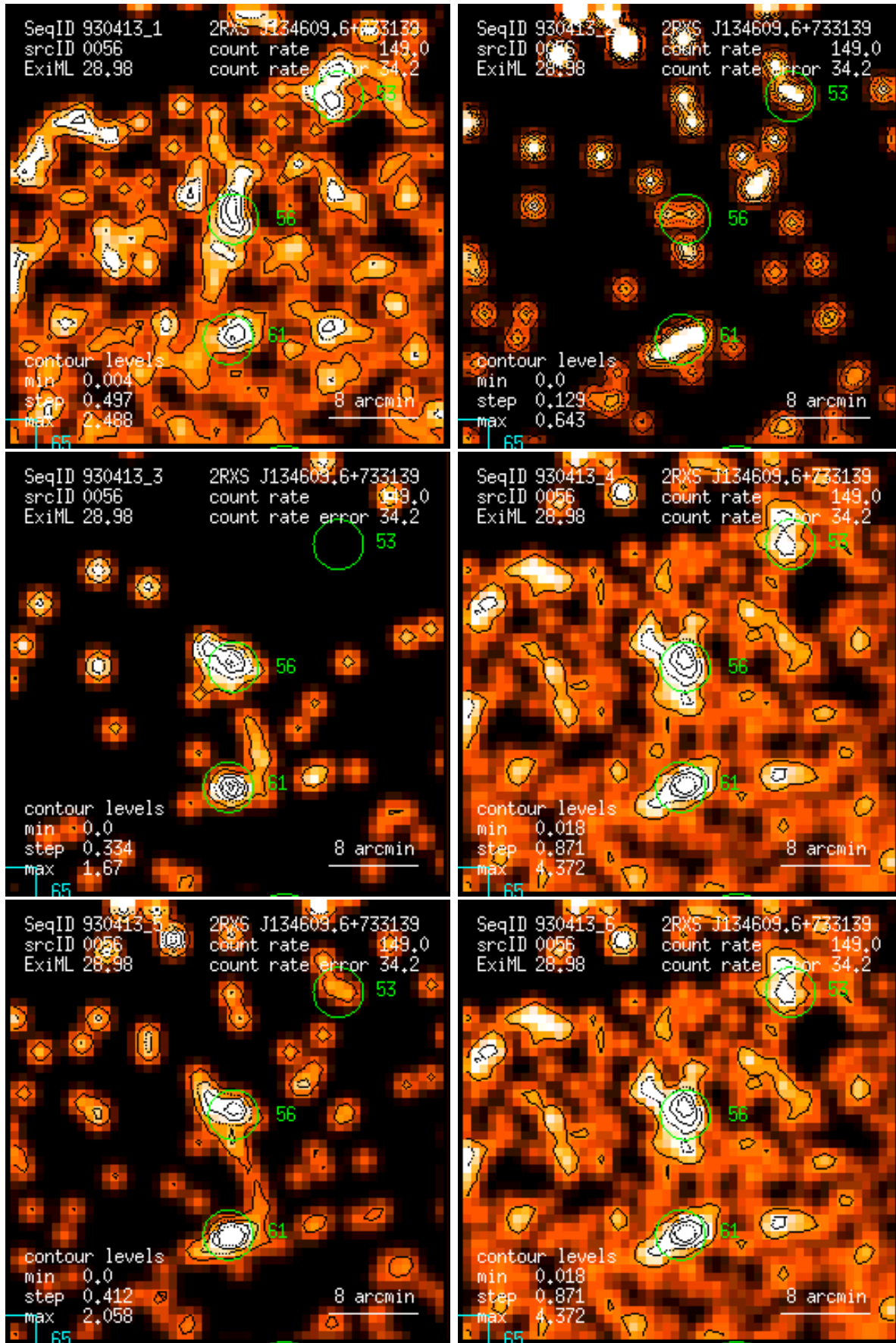
Figure 56: RASS 930413: detection 0056: band rate images, Gaussian filter: (1) PSPC channels 11 – 41, (2) 52 – 90, (3) 91 – 201, (4) 11 – 235, (5) 52 – 201, (6) 11 – 201. Broad band rates in counts/ks. Band rate contour levels in counts/ks/arcmin 2 .
