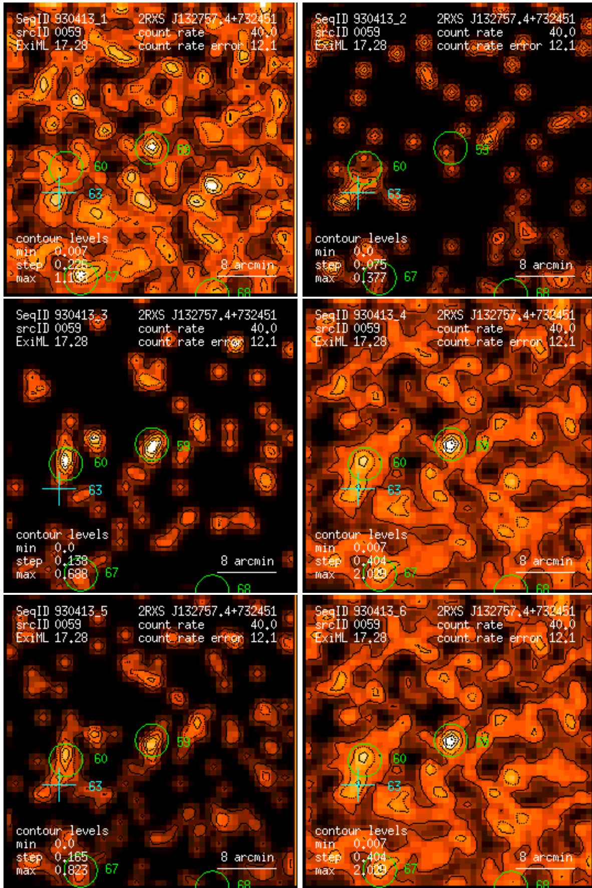
Figure 59: RASS 930413: detection 0059: band rate images, Gaussian filter: (1) PSPC channels 11 – 41, (2) 52 – 90, (3) 91 – 201, (4) 11 – 235, (5) 52 – 201, (6) 11 – 201. Broad band rates in counts/ks. Band rate contour levels in counts/ks/arcmin 2 .
