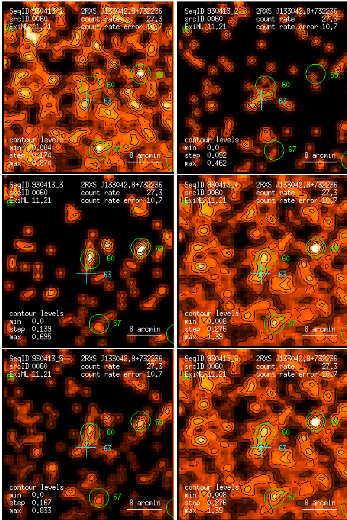
Figure 60: RASS 930413: detection 0060: band rate images, Gaussian filter: (1) PSPC channels 11 – 41, (2) 52 – 90, (3) 91 – 201, (4) 11 – 235, (5) 52 – 201, (6) 11 – 201. Broad band rates in counts/ks. Band rate contour levels in counts/ks/arcmin 2 .
