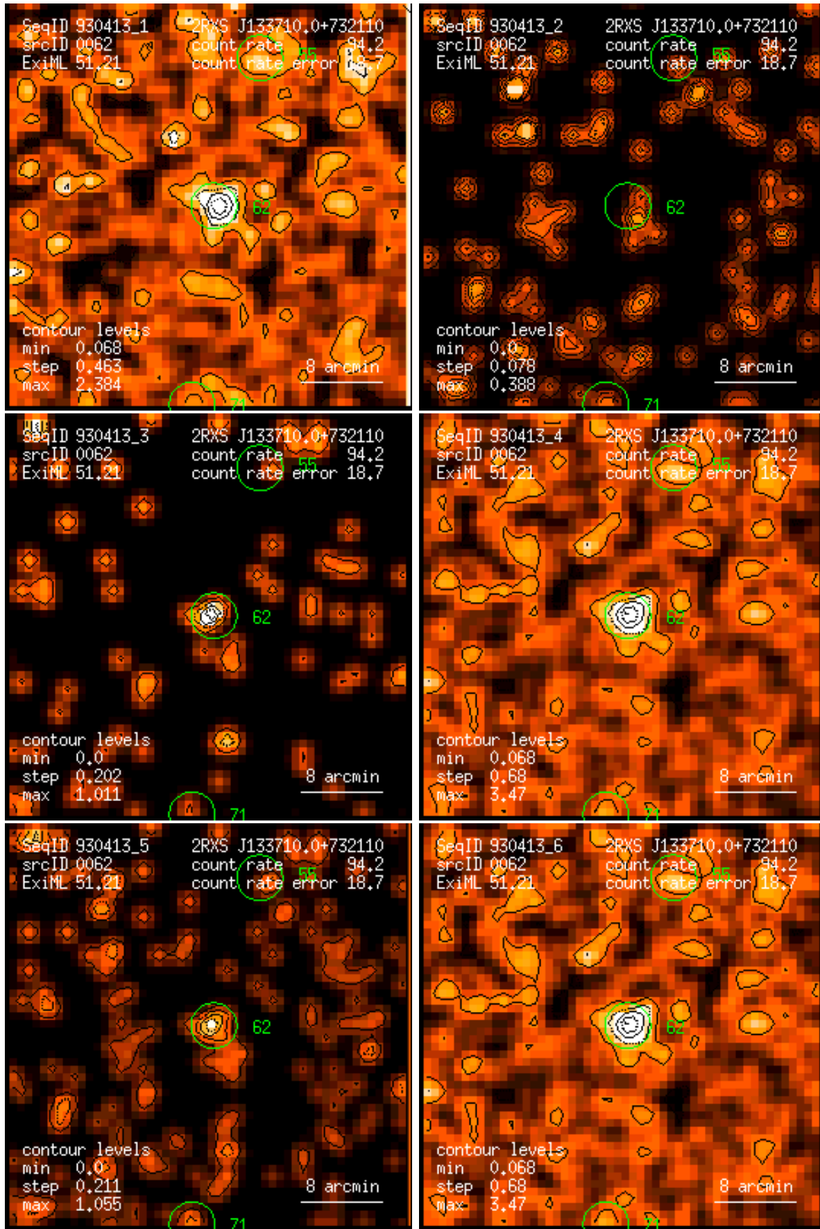
Figure 62: RASS 930413: detection 0062: band rate images, Gaussian filter: (1) PSPC channels 11 – 41, (2) 52 – 90, (3) 91 – 201, (4) 11 – 235, (5) 52 – 201, (6) 11 – 201. Broad band rates in counts/ks. Band rate contour levels in counts/ks/arcmin 2 .
