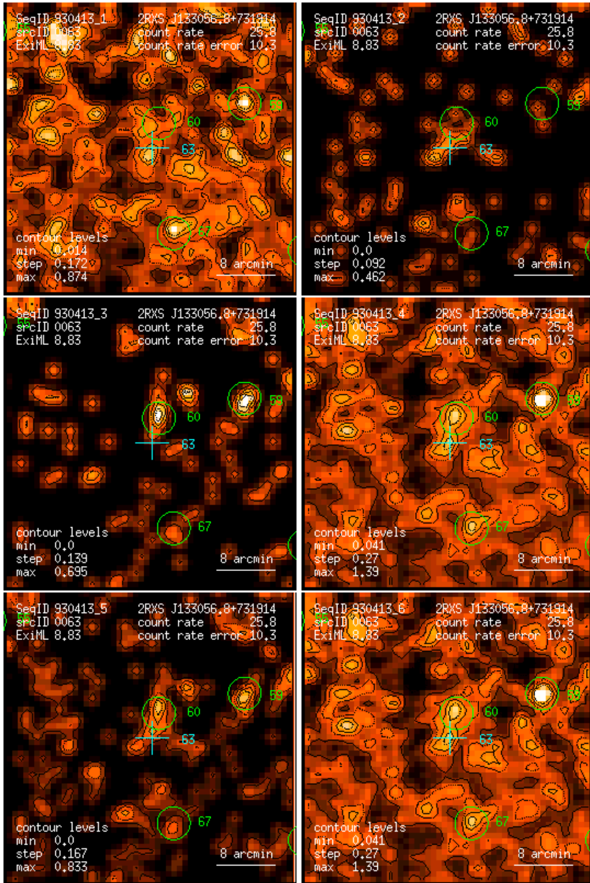
Figure 63: RASS 930413: detection 0063: band rate images, Gaussian filter: (1) PSPC channels 11 – 41, (2) 52 – 90, (3) 91 – 201, (4) 11 – 235, (5) 52 – 201, (6) 11 – 201. Broad band rates in counts/ks. Band rate contour levels in counts/ks/arcmin 2 .
